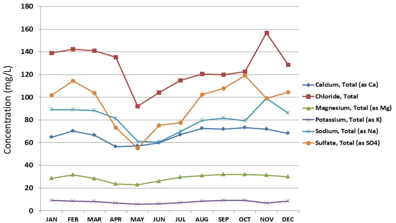
Figure BLANK: Average calendar month maximum concentrations of various parameters measured in the effluent from Hibbing WWTP
