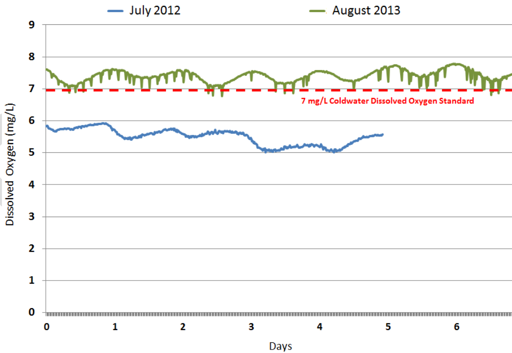
Figure BLANK: Results from two continuous dissolved oxygen surveys at biological monitoring station 09LS062
