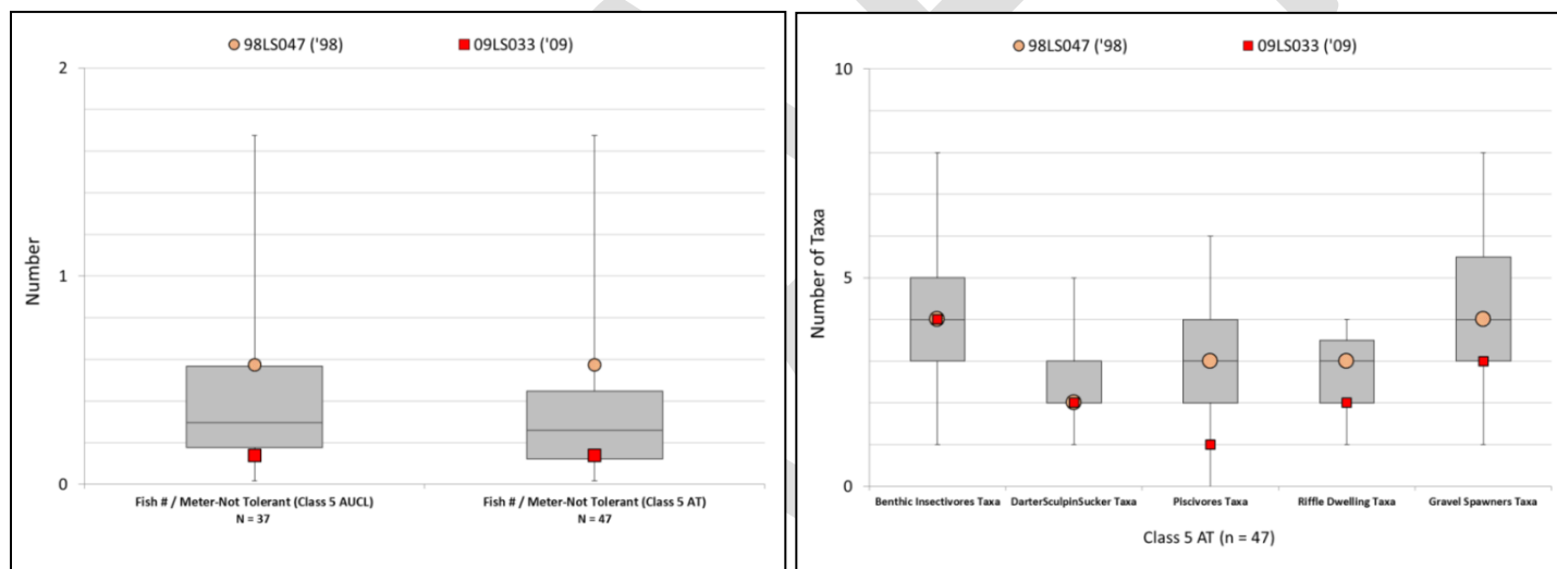
Figure BLANK: (Left) Non-tolerant fish/meter in Sand Creek compared to high quality Class 5 SLRW stations. (Right) Number of fish taxa for various categories in Sand Creek compared to Class 5 SLRW stations above the impairment threshold
