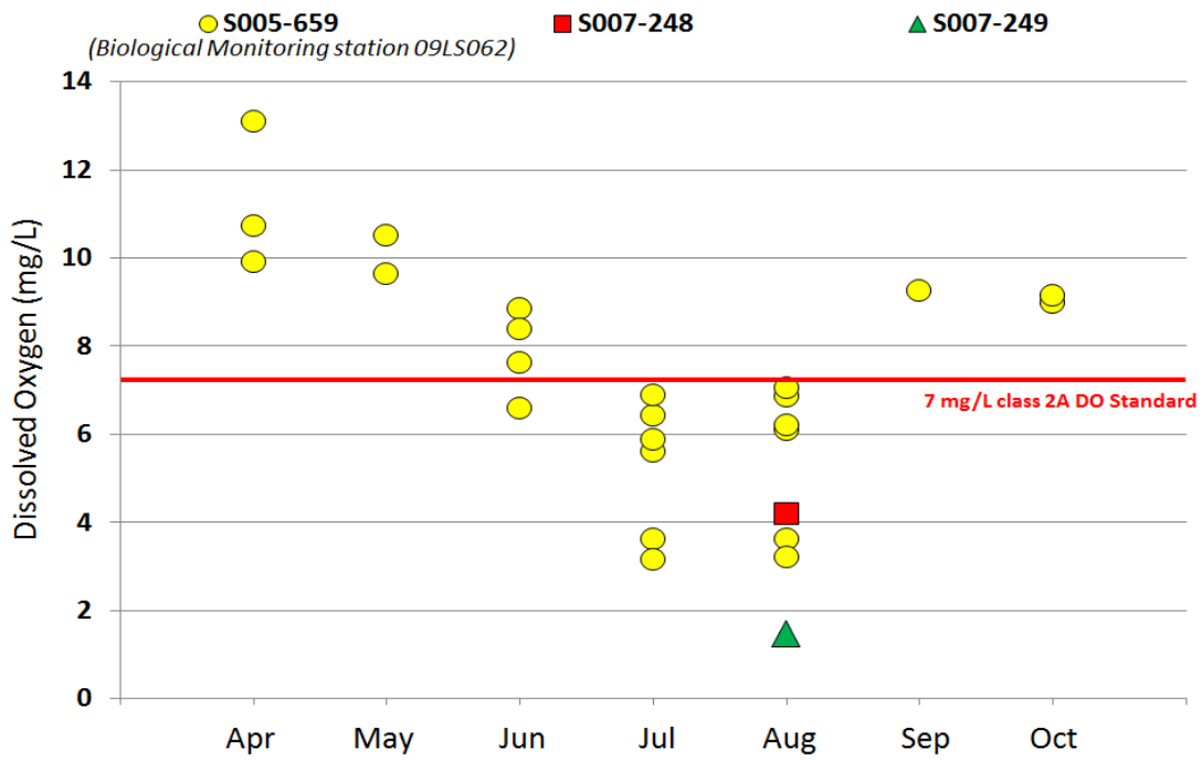
Figure BLANK: Instantaneous measurements of dissolved oxygen by monitoring station and calendar month.
