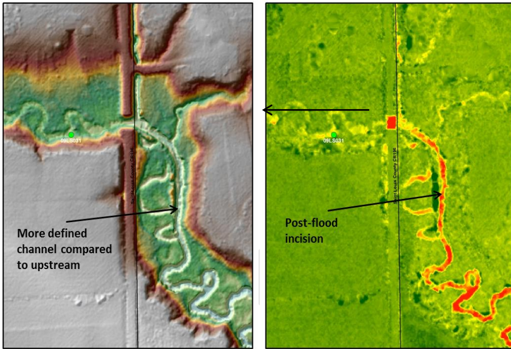
Figure BLANK (left): Two LiDAR images of Skunk Creek 09LS031, one showing an incised channel, the other showing evidence of degradation following the June 2012 flood (scale: green → yellow → red = little change → moderate change → severe change).
