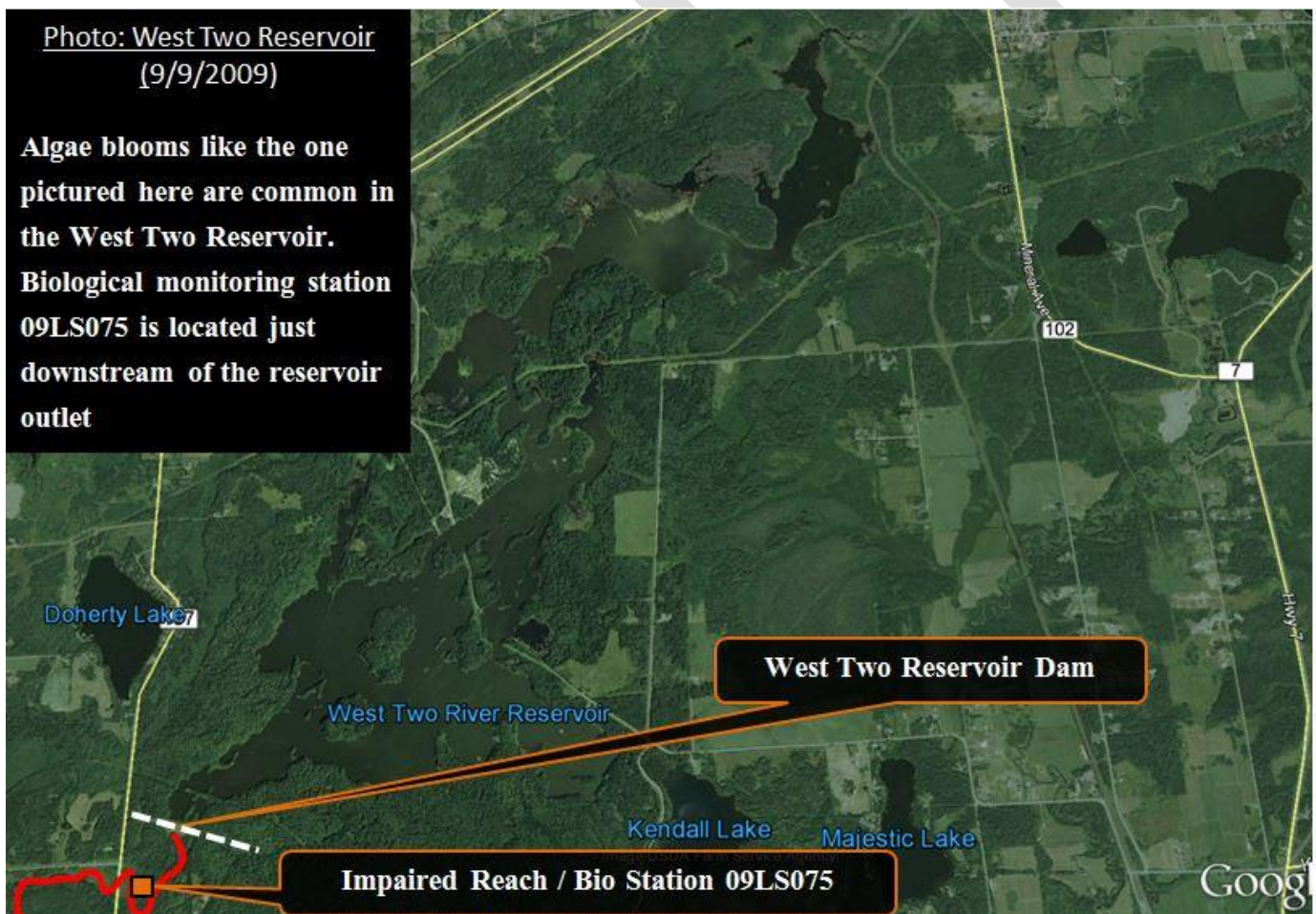
Figure BLANK: Aerial photo showing algae bloom in the West Two Reservoir, and location of biological monitoring station 09LS075 in relation to the reservoir outlet
