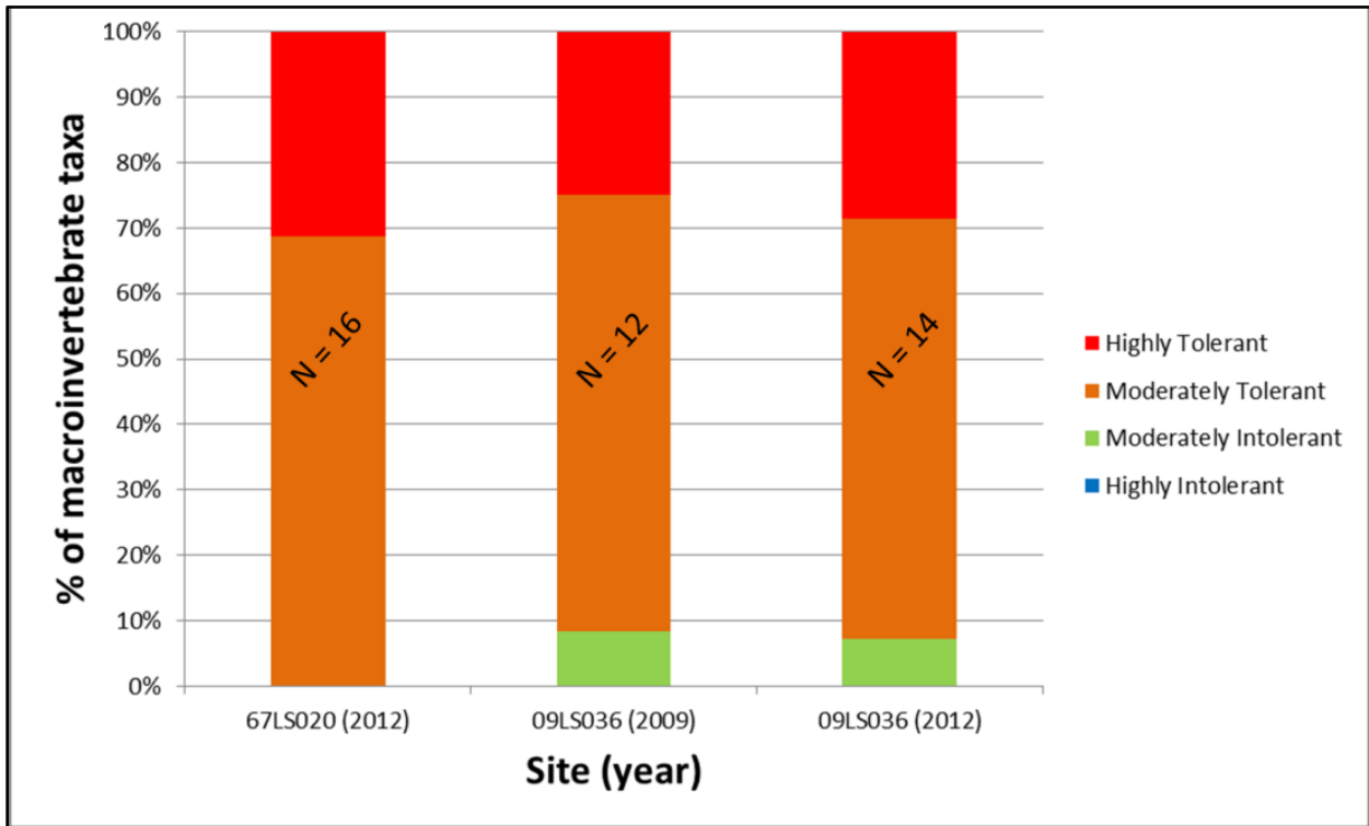
Figure BLANK: TSS tolerance of macroinvertebrate assemblages by site in Stony Creek (n = number of taxa)
