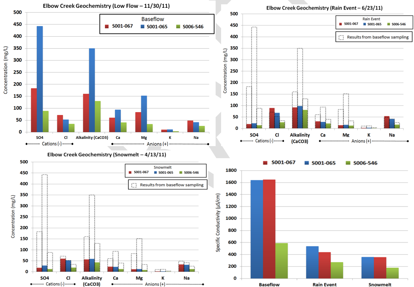
Figure BLANK: Geochemistry sampling results for Elbow Creek during baseflow (upper left), rain event flow (upper right), and snowmelt flow (lower left). Specific conductivity readings for the three monitoring events are shown (lower right)
