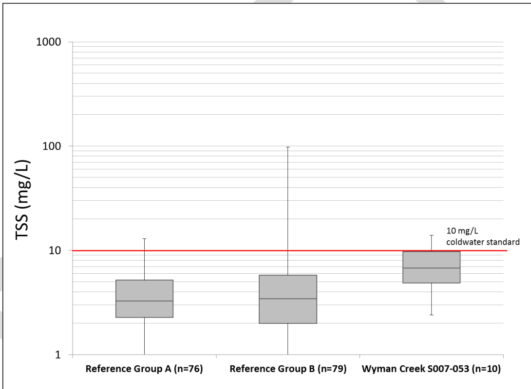
Figure BLANK: Box plots of TSS values for Wyman Creek and reference streams
