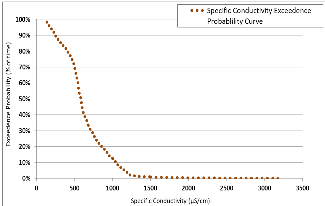
Figure 59: Exceedance probability curve for the 2006 specific conductivity data set from station S004-952
