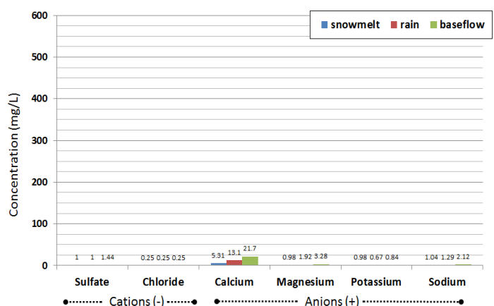
Figure BLANK: Concentrations of major cations and anions observed in Spring Mine Creek (left; impacted) and Bear Creek (right; undisturbed reference).
