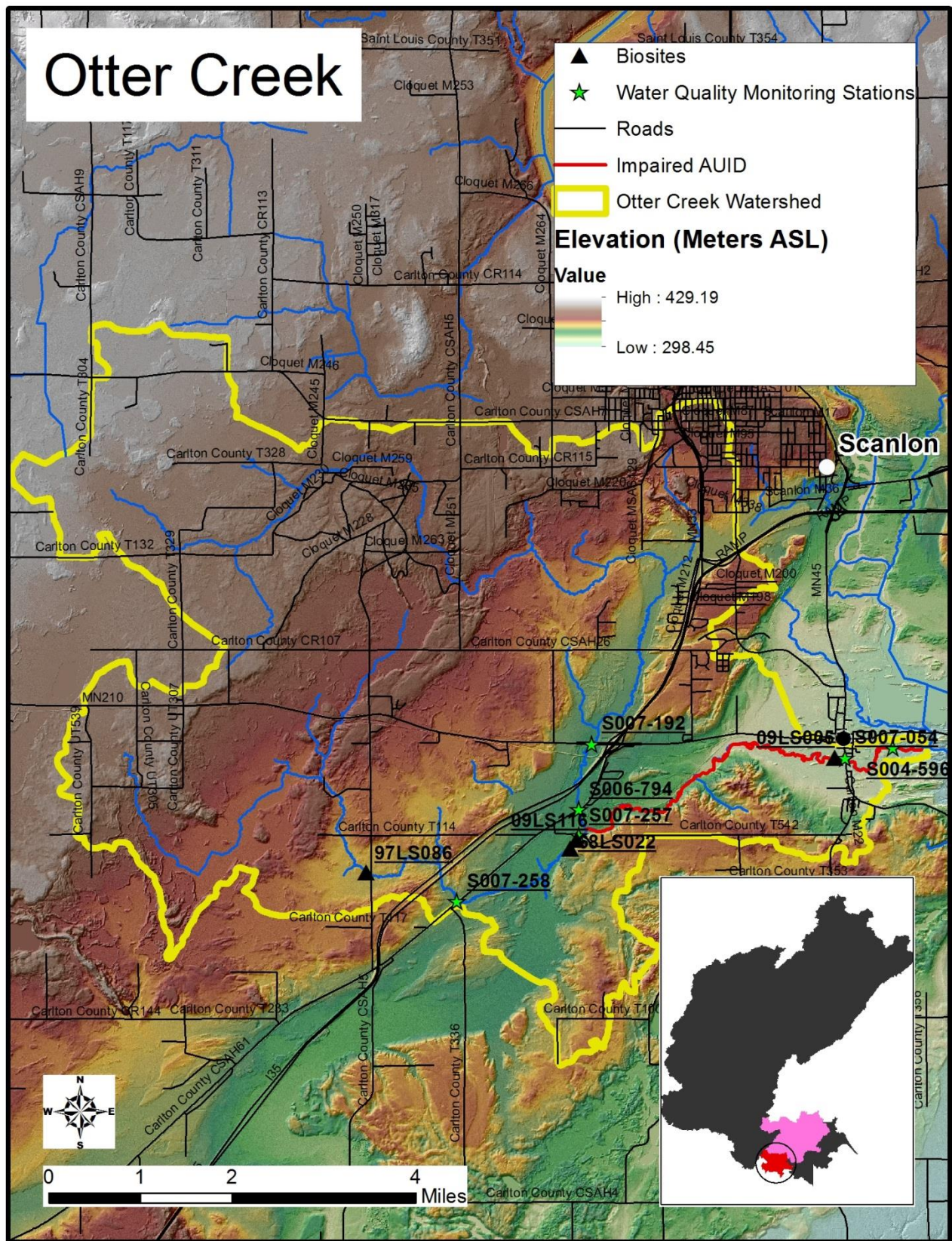
Figure xx: Map of Otter Creek watershed and impaired stream reach
