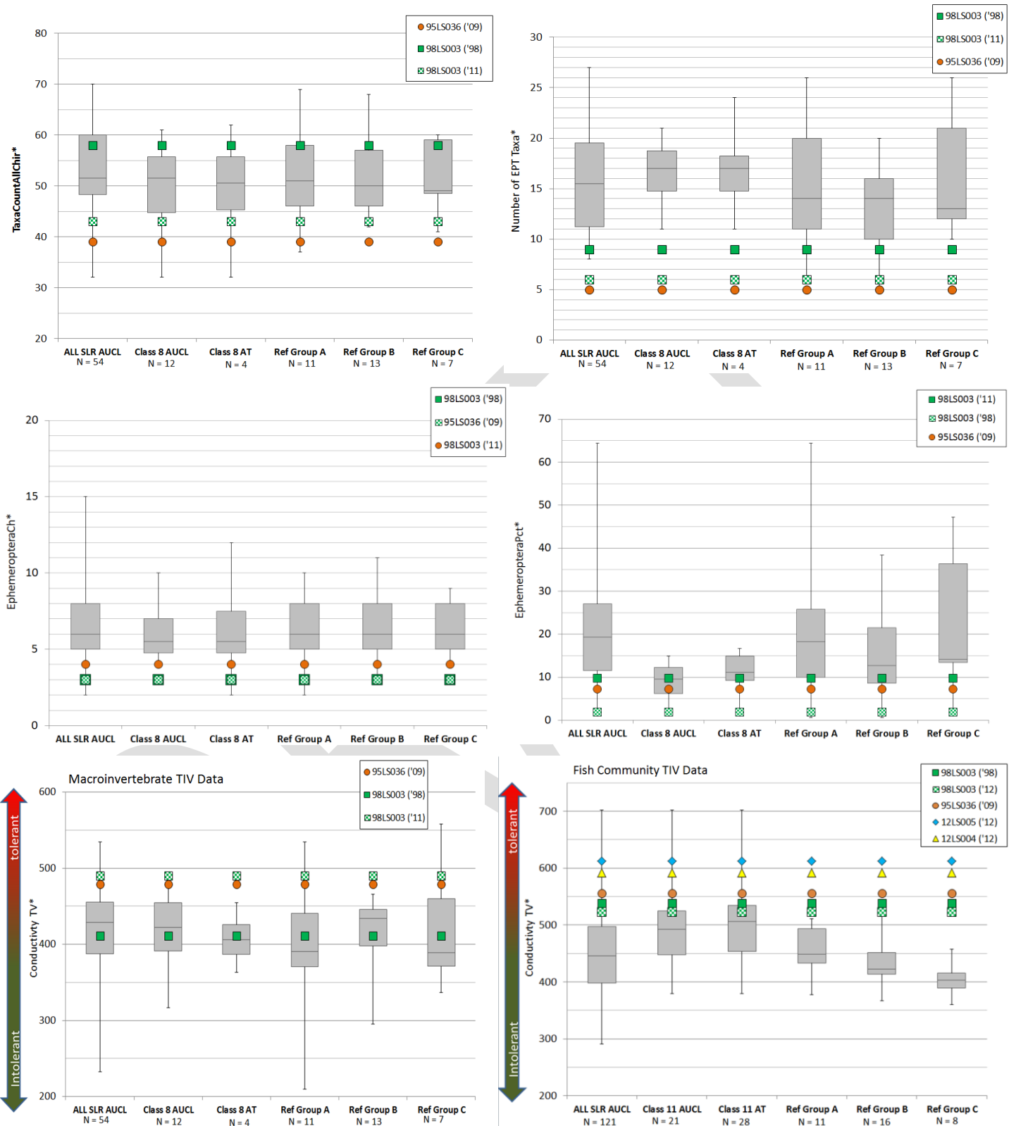
Figure 62: Collection of box-plot distribution graphs comparing biological response data from Kingsbury Creek to results from SLRW reference streams. (* See table BLANK for acronyms)
