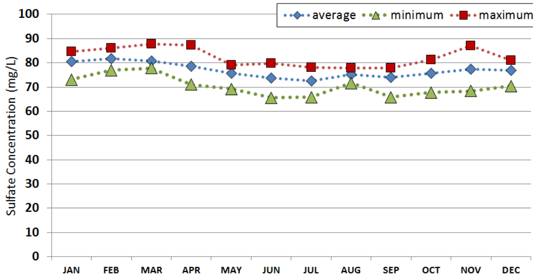
Figure BLANK: Sulfate concentrations of mine pit dewatering effluent discharged to Wyman Creek
