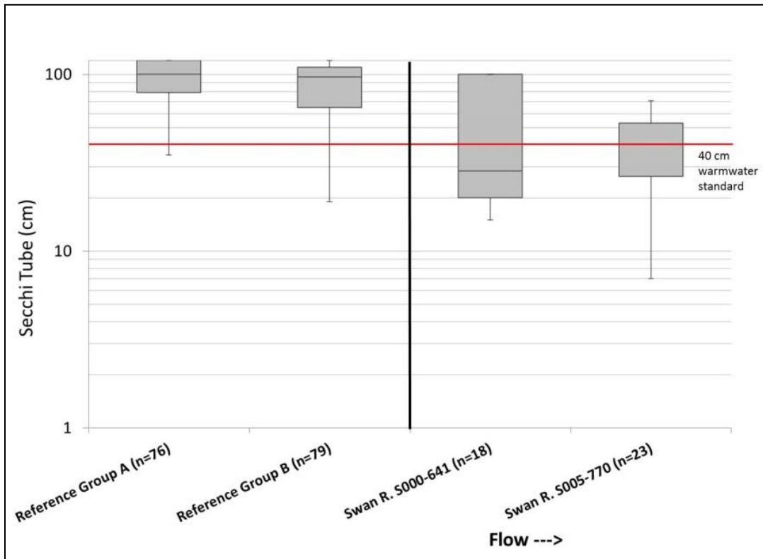
Figure BLANK: Box plots of Secchi Tube values for the Swan River and reference streams (see section BLANK for reference streams)
