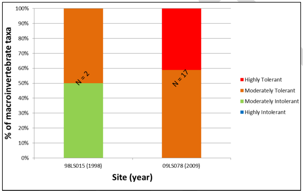
Figure BLANK: TSS tolerance of the macroinvertebrate assemblage in Manganika Creek (n = number of taxa)
