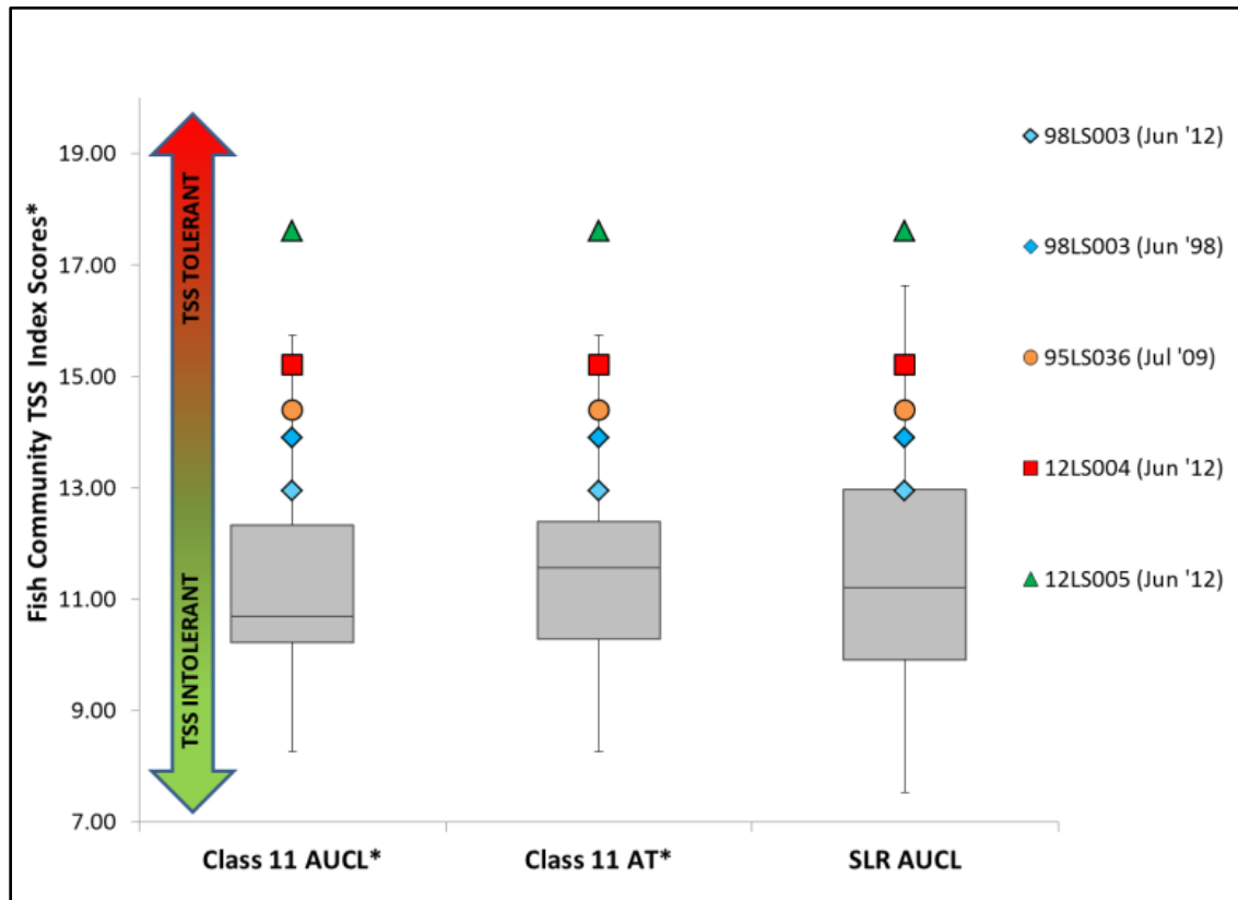
Figure 51: Fish community TSS TIVs for Kingsbury Creek, compared to unimpaired streams
