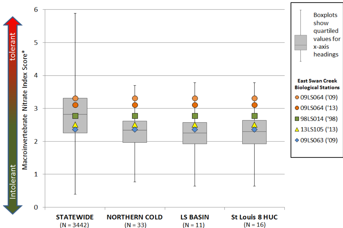
Figure BLANK: Macroinvertebrate community nitrate tolerance indicator values (NTIV) for East Swan Creek monitoring stations compared to results from statewide and regional sites.
