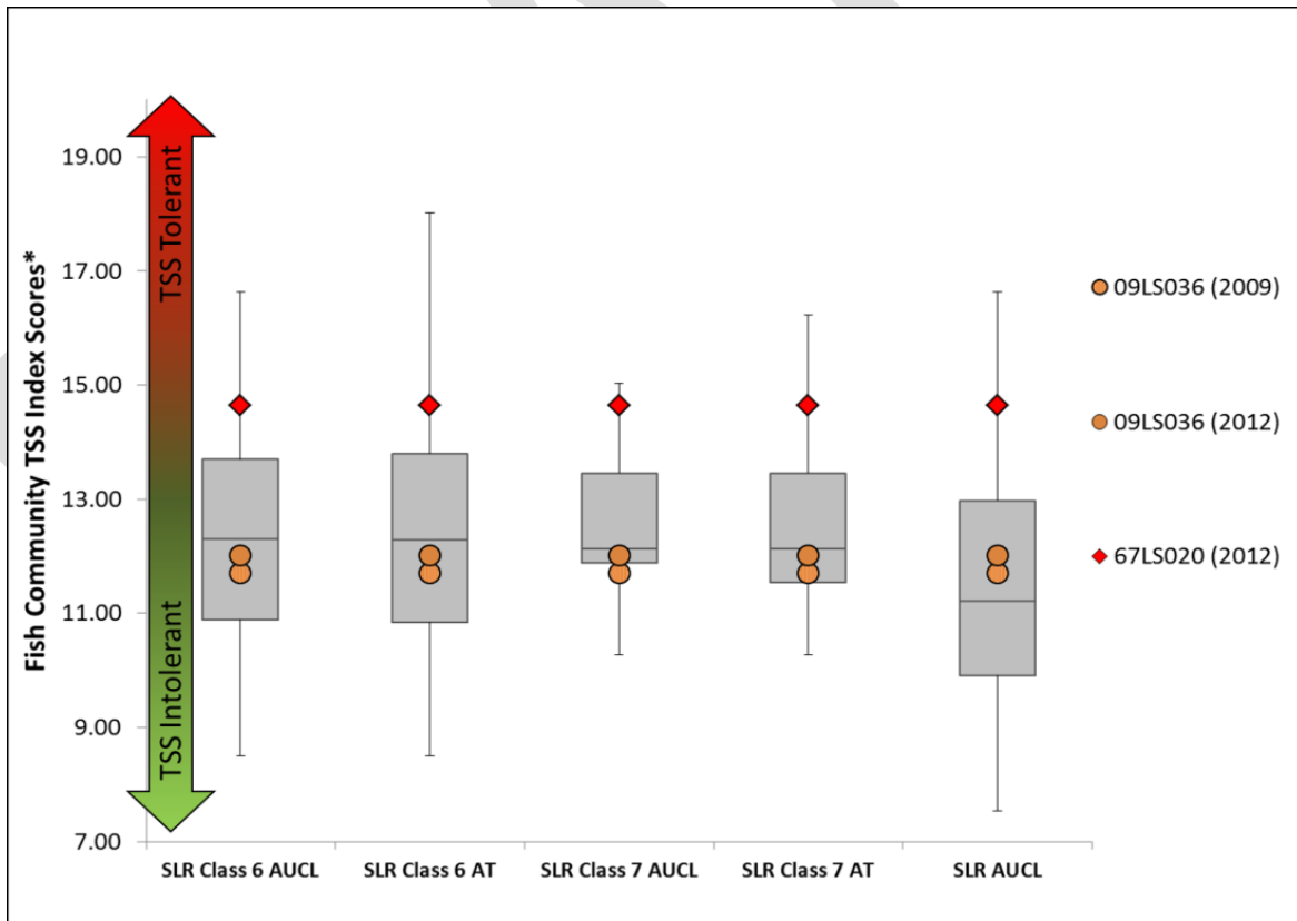
Figure BLANK: Fish community TSS TIVs for Stony Creek, compared to unimpaired streams
