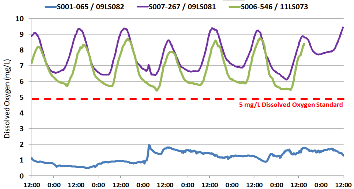
Figure BLANK: Continuous DO data collected at three Elbow Creek biological monitoring stations in August 2012
