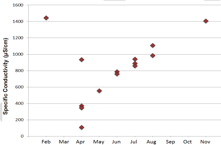
Figure BLANK: Instantaneous specific conductivity measurements collected at biological monitoring station 09LS101 by month. Data were collected between 2011 – 2014.
