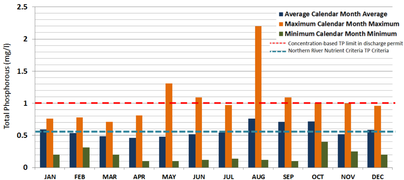
Figure BLANK: Total phosphorous concentrations of Virginia WWTP effluent discharged to Manganika Creek
