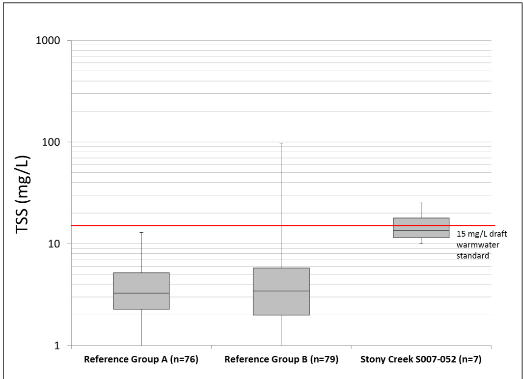
Figure BLANK: Box plots of TSS values for Stony Creek and reference streams
