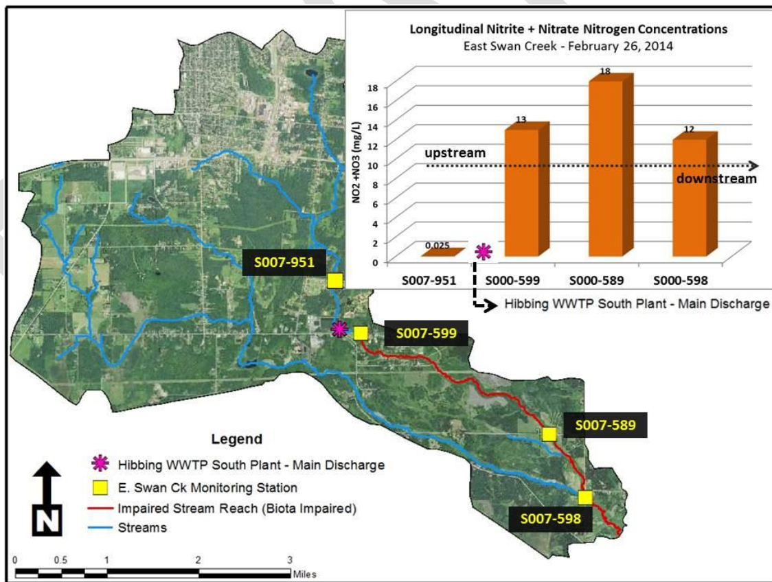
Figure BLANK: Nitrate concentrations observed in East Swan Creek during a February 2014 longitudinal sampling event
