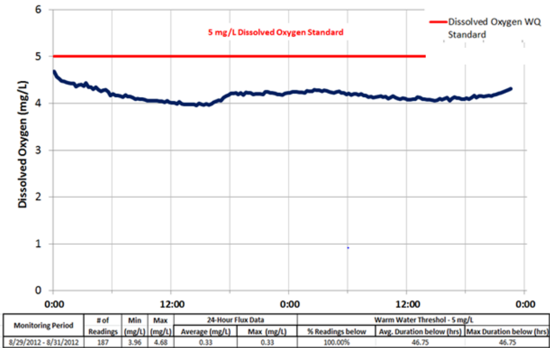
Figure BLANK: Results from continuous monitoring at biological monitoring station 97LS034 over a 2-day period in August 2012
