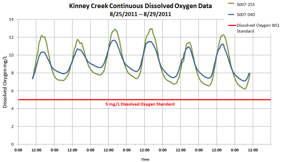
Figure BLANK: Continuous dissolved oxygen data from two Kinney Creek biological monitoring stations in August 2011
