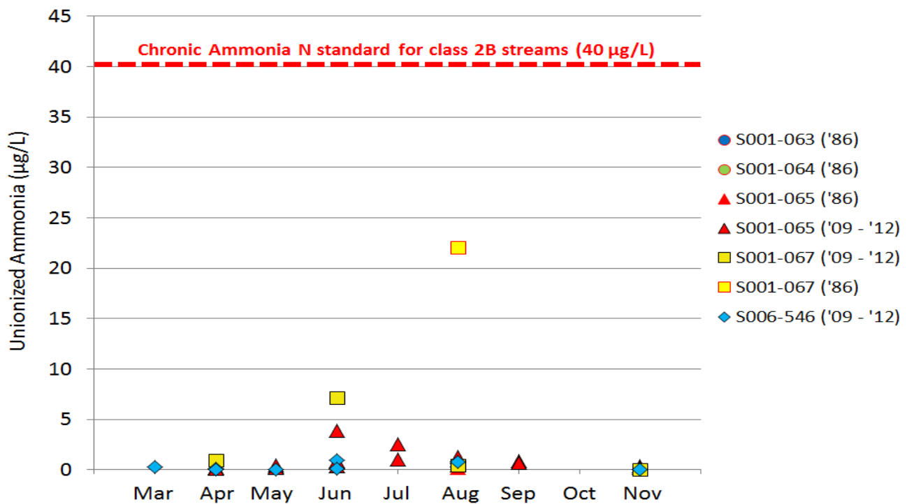
Figure BLANK: Unionized ammonia nitrogen results observed at Elbow Creek monitoring stations, arranged by month
