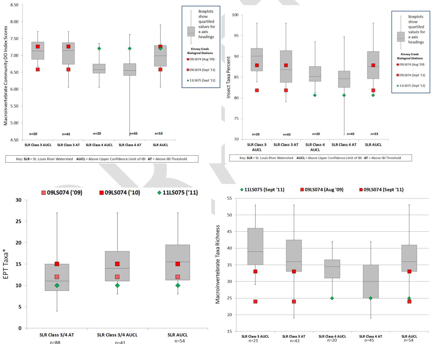
Figure BLANK: Comparison of results for several macroinvertebrate metrics between Kinney Creek stations and non-impaired SLRW reference stations: macroinvertebrate community DO tolerance indicator values (TIV) (top left), % Insect Taxa (top right); EPT Taxa Richness (lower left); overall macroinvertebrate taxa richness (lower right)
