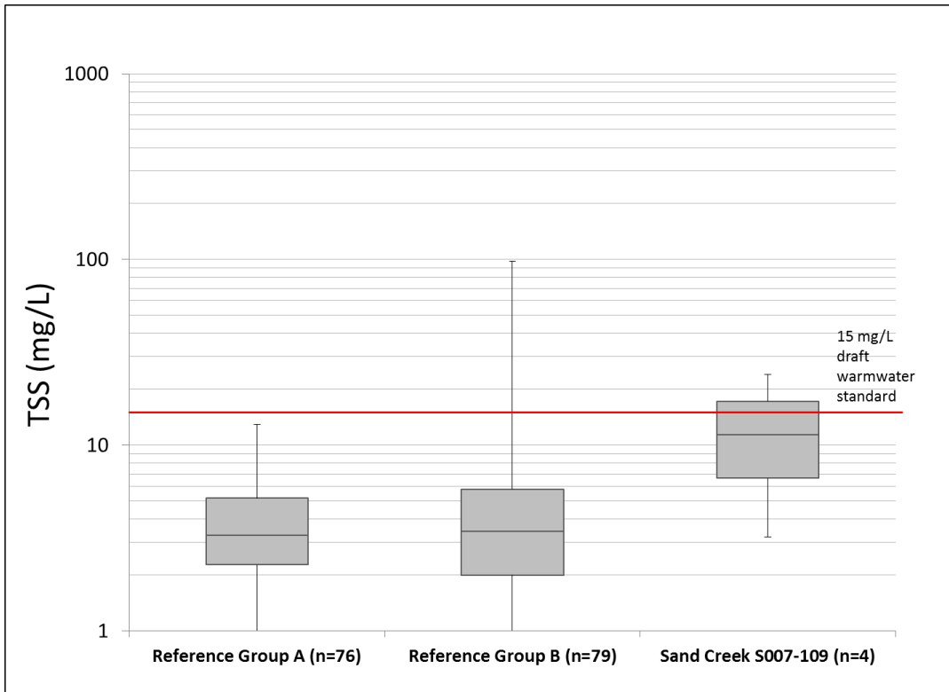
Figure BLANK: Box plots of TSS values for Sand Creek compared to reference streams (see section BLANK).
