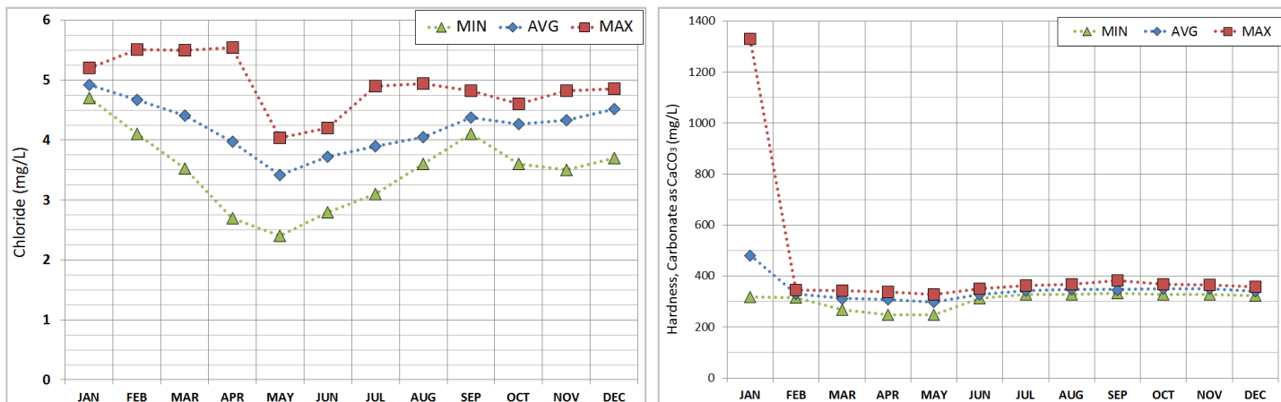
Figure BLANK: Monitoring data for chloride and total hardness associated with permitted discharge MN0042536-SD-33 to Spring Mine Creek
