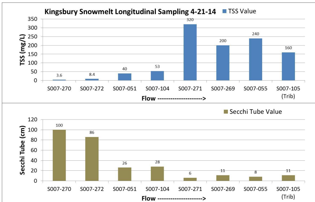
Figure 41: TSS and Secchi Tube results from a 4/21/2014 snowmelt sampling event on Kingsbury Creek
