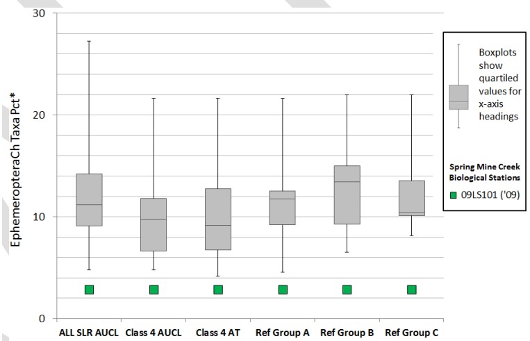
Figure BLANK: Ephemeroptera taxa richness (left) and Ephemeroptera taxa percent (right) from Spring Mine Creek compared to high quality reference stations.
