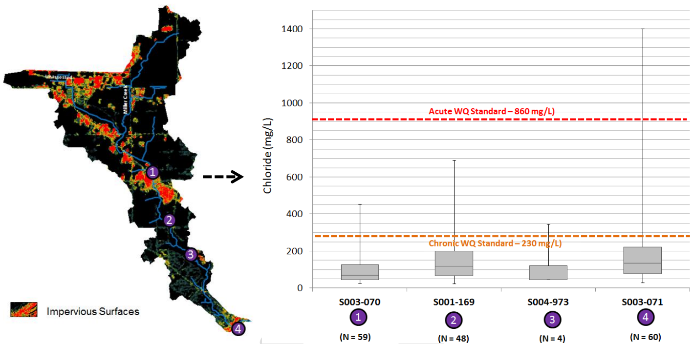
Figure 77: Box plots of all chloride sampling results for Miller Creek arranged by monitoring station
