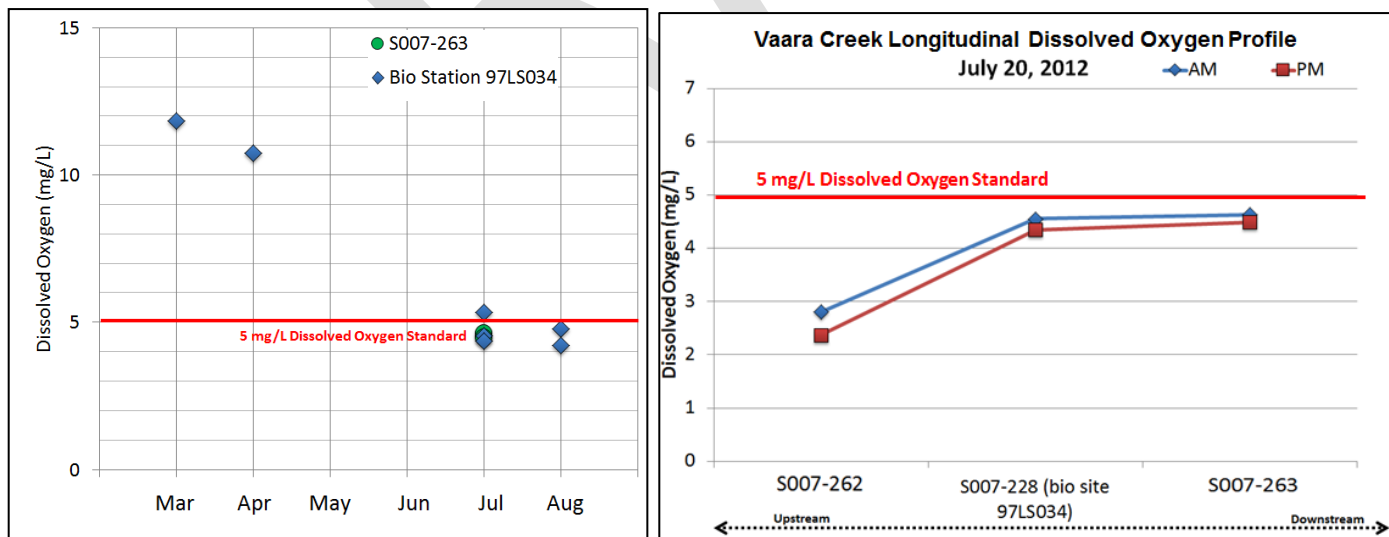
Figure BLANK: (Left) Results from spot measurements of dissolved oxygen sorted by calendar month.
