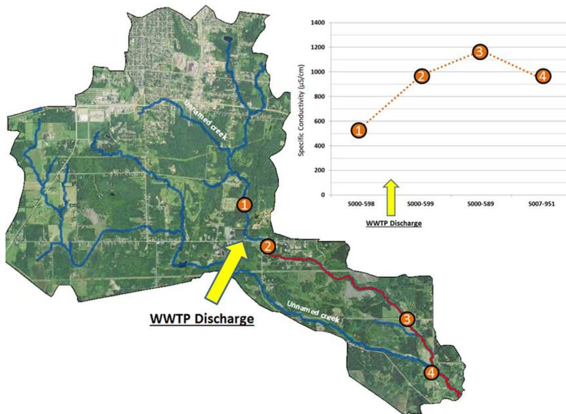
Figure BLANK: Longitudinal measurements of specific conductivity from East Swan Creek collected in February 2014
