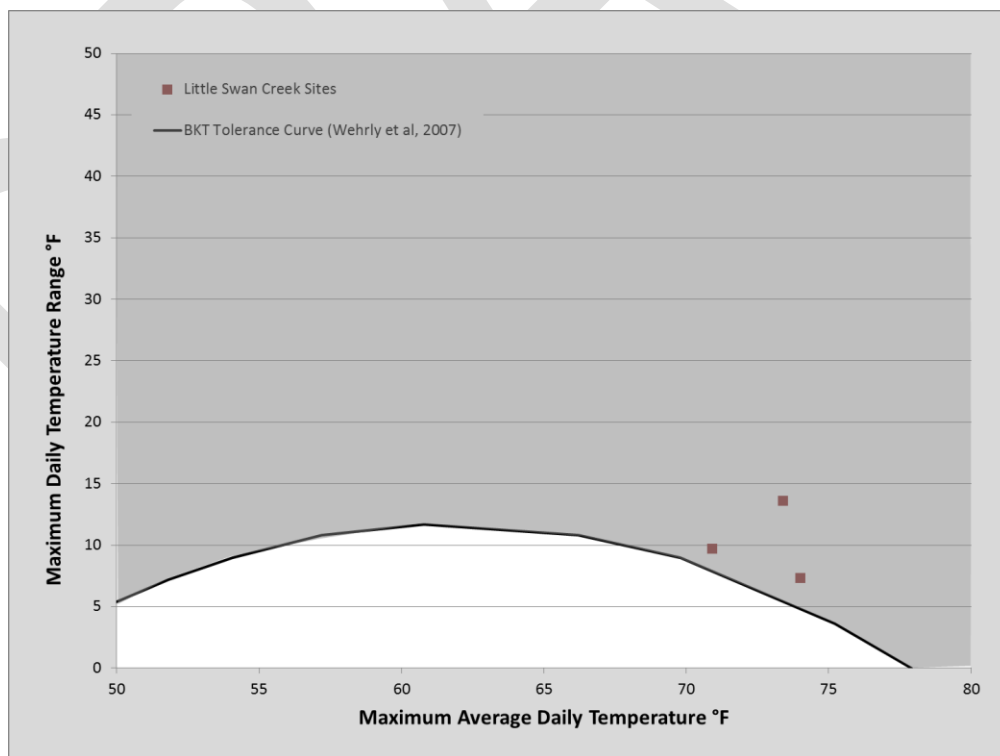
Figure BLANK: Maximum daily temperature and maximum temperature fluctuation recorded on Little Swan Creek
