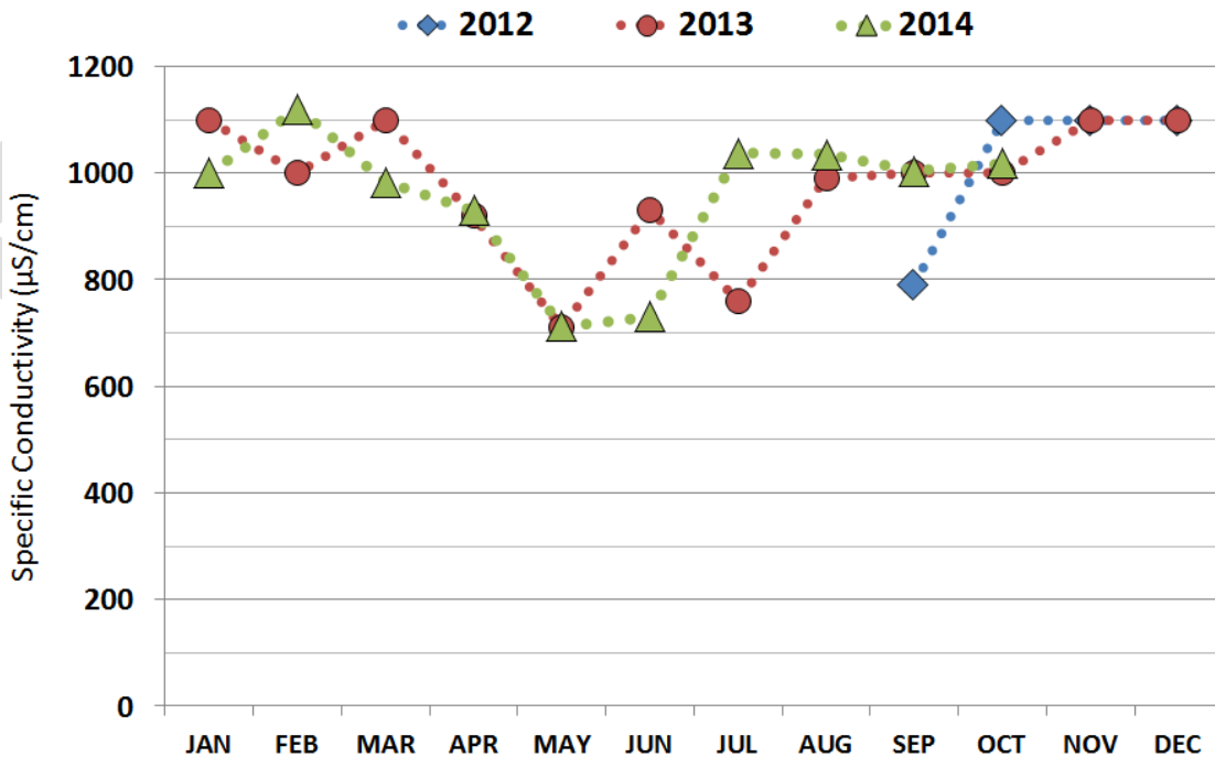
Figure BLANK: Monthly maximum specific conductivity values of effluent discharged from Hibbing WWTP to East Swan Creek
