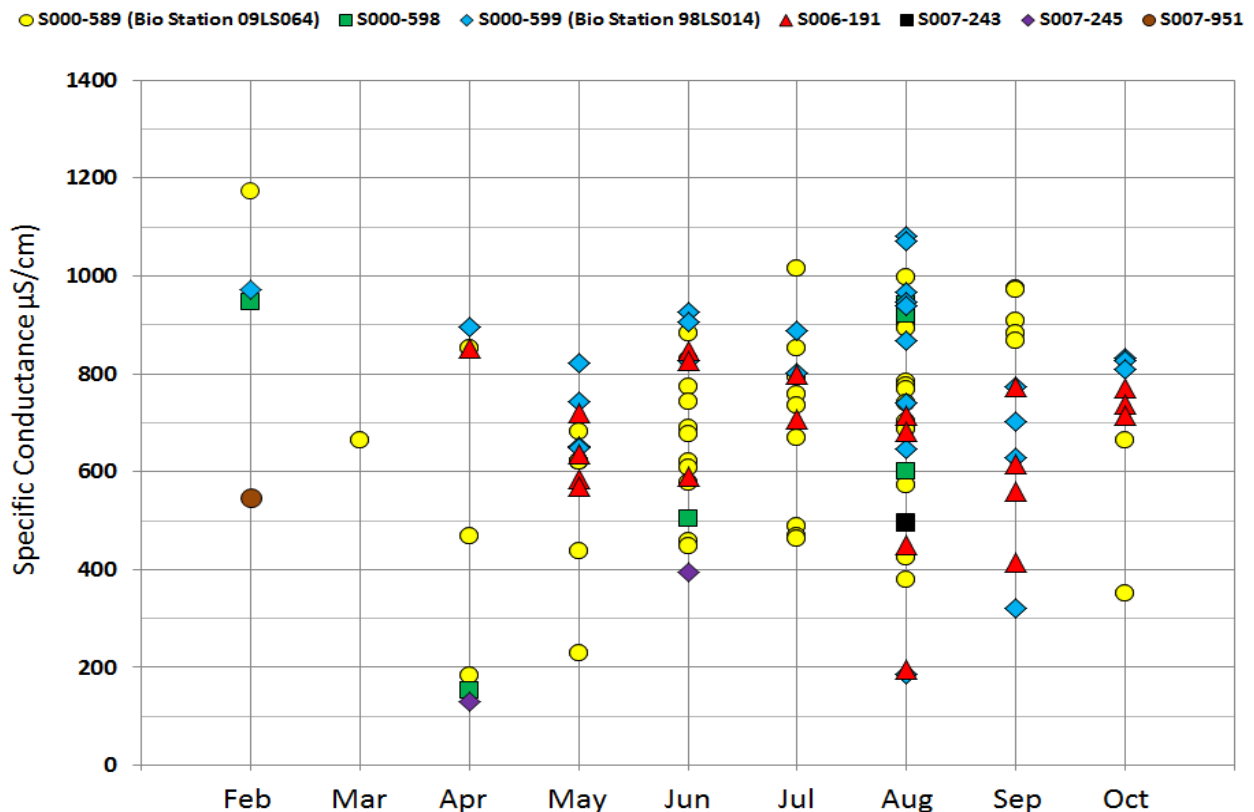
Figure BLANK: Point measurements of specific conductivity collected from East Swan Creek by monitoring station and calendar month
