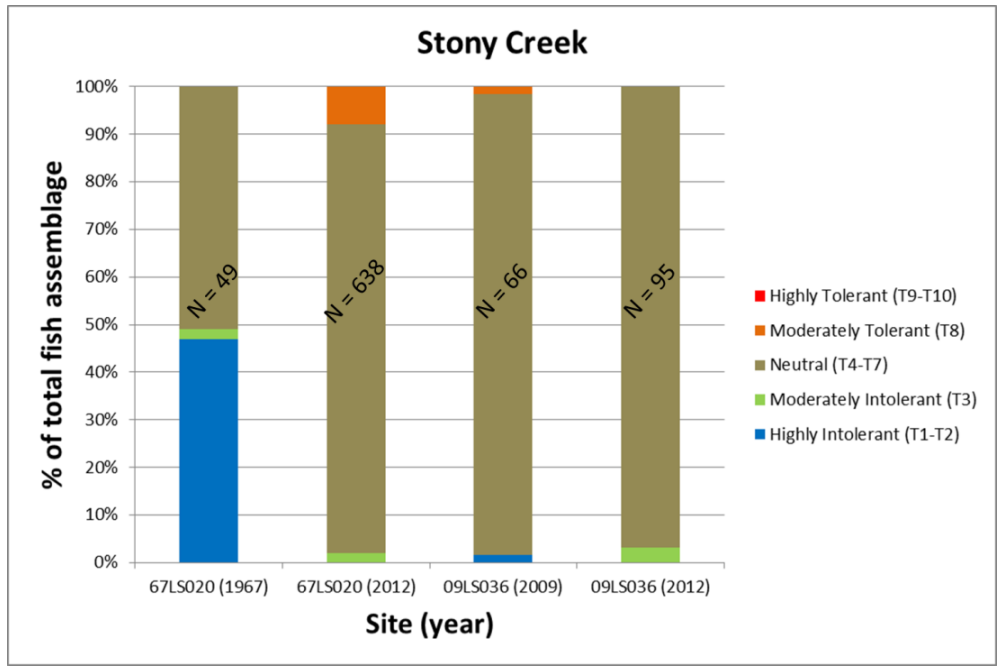
Figure BLANK: TSS tolerance of fish assemblages by site in Stony Creek (n = number of fish)
