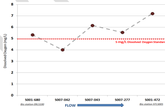
Figure BLANK: Longitudinal dissolved oxygen data from upper Embarrass River monitoring stations (August 2012)
