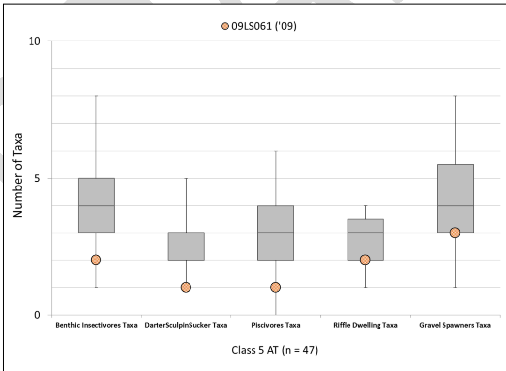
Figure BLANK: Number of fish taxa for various categories observed at Swan River station 09LS061 compared to Class 5 SLRW stations above the impairment threshold
