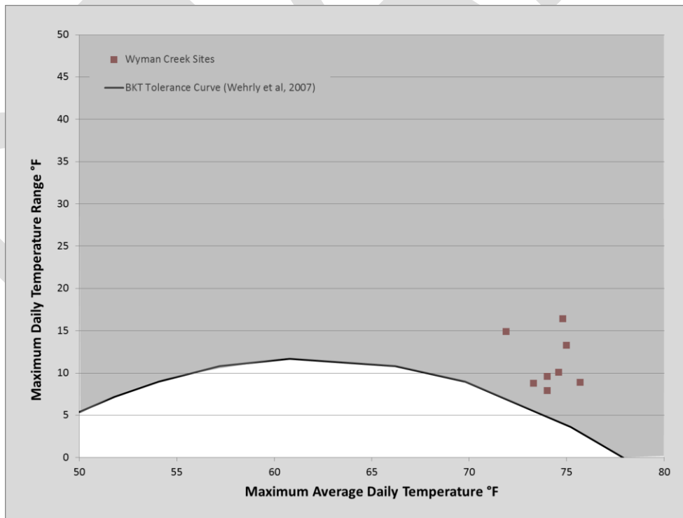
Figure BLANK: Maximum daily temperature and maximum temperature fluctuation recorded in Wyman Creek
