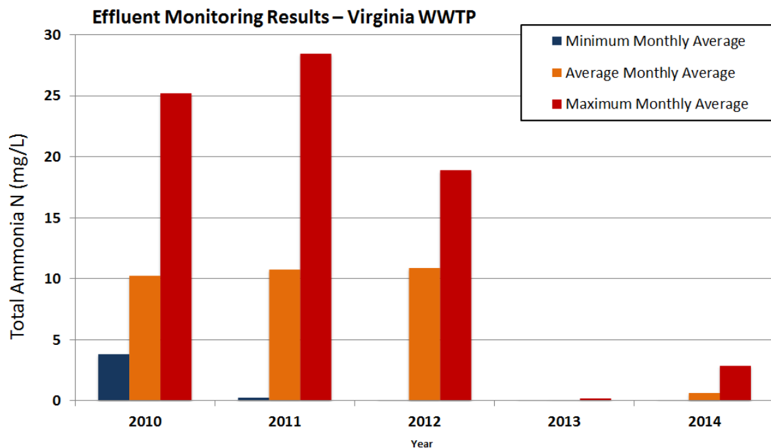
Figure BLANK: Effluent monitoring results for total ammonia discharged from the Virginia WWTP to Manganika Creek
