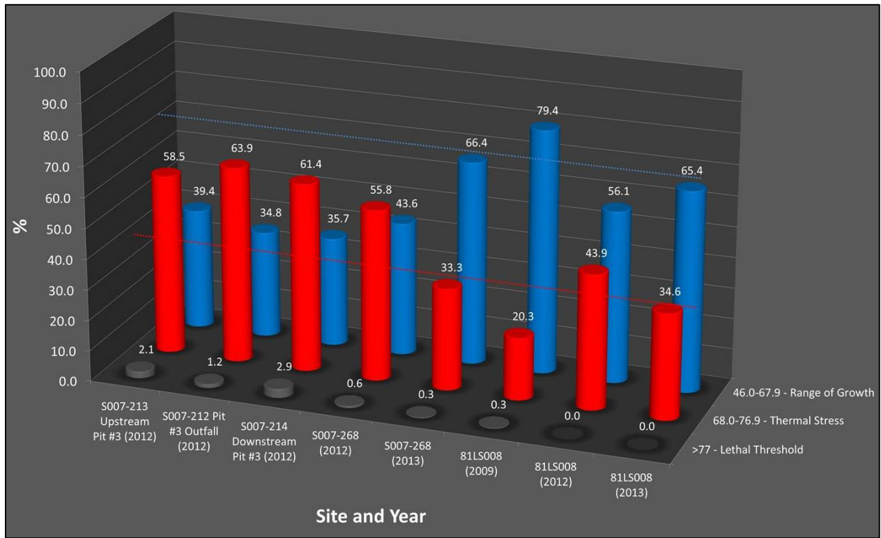
Figure BLANK: Percentage of time spent in BKT growth, stress and lethal ranges
