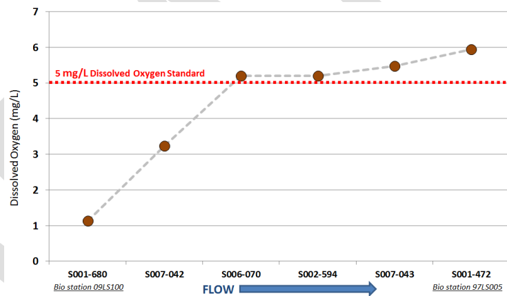
Figure BLANK: Longitudinal dissolved oxygen data from upper Embarrass River monitoring stations (August 2011)
