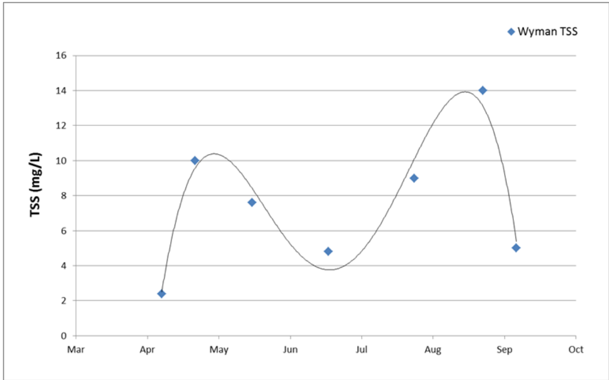
Figure BLANK: TSS results from Wyman Creek by calendar month
