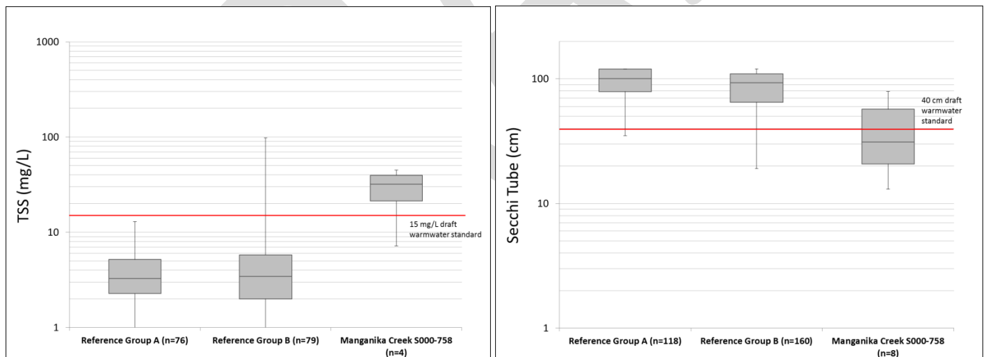
Figure BLANK: Box plots of TSS and s-tube results for Manganika Creek and SLRW reference streams
