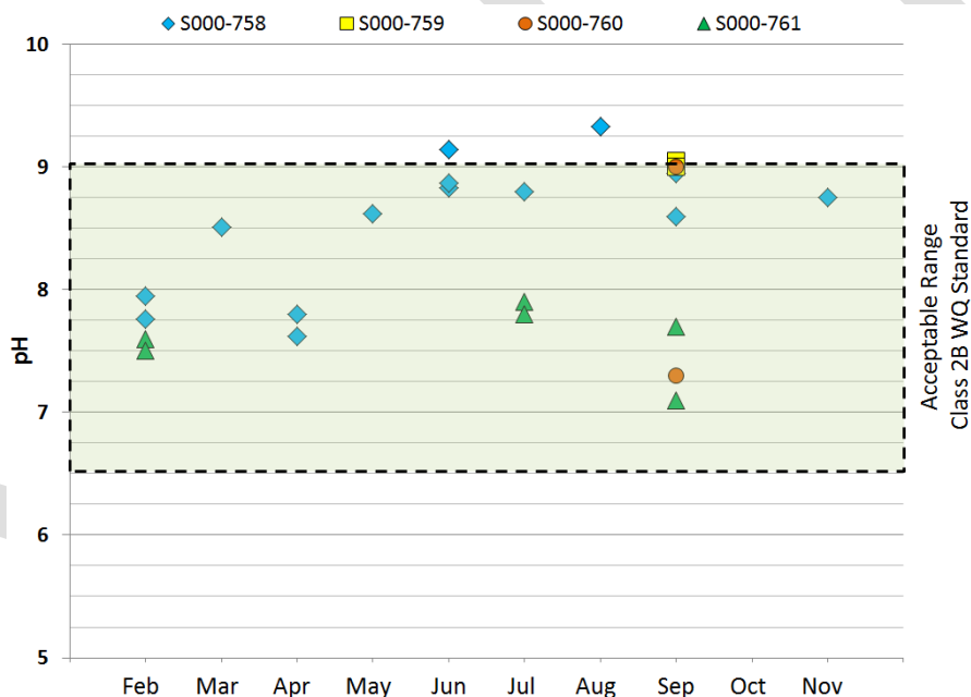
Figure BLANK: pH data from Manganika Creek arranged by calendar month and monitoring stations,
