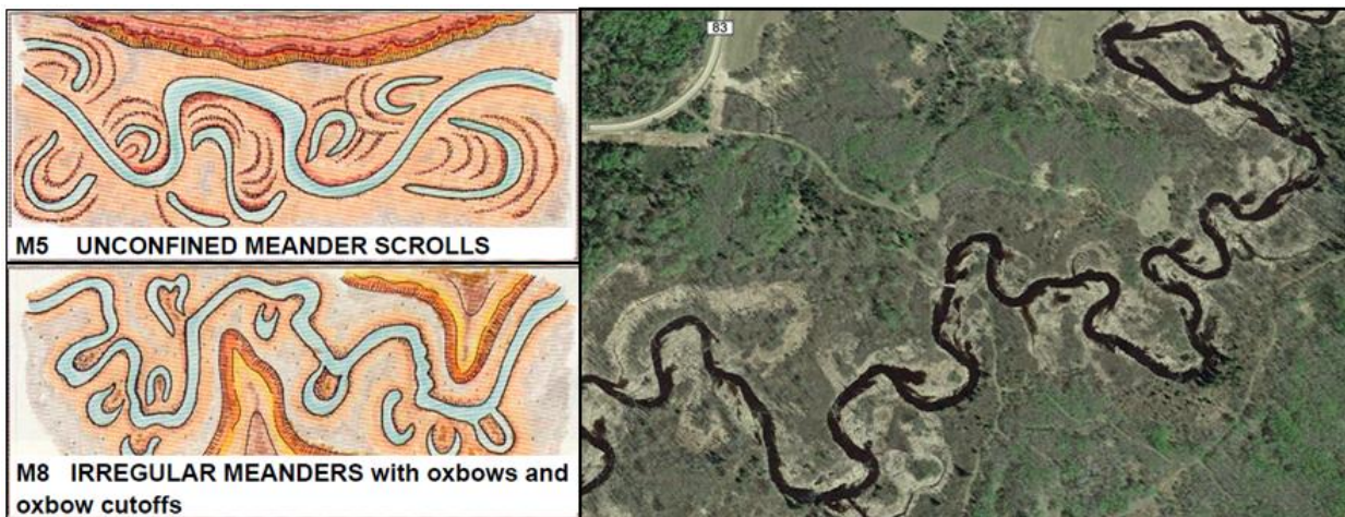
Figure 2: (Left) Meander patterns that apply to Stony Creek (from Rosgen 2006). (Right) Aerial photo of Stony Creek showing irregular meander pattern, oxbows, and oxbow cutoffs (see upper right of photo for large oxbow cutoff)
