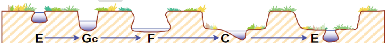
Figure BLANK: Ely Creek channel evolution scenario (from the River Stability Field Guide, Rosgen 2008)
