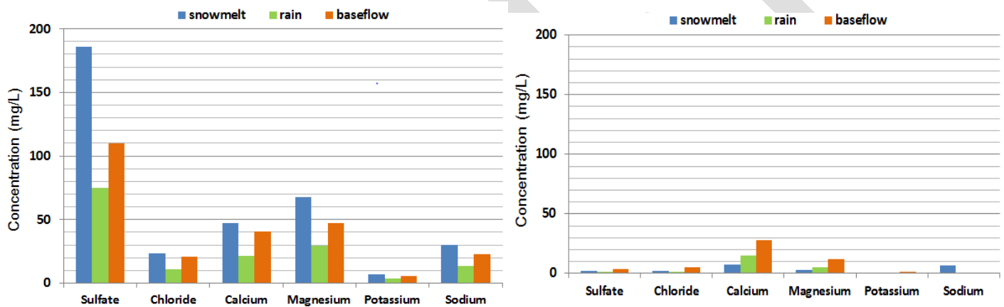
Figure BLANK and BLANK: Concentrations of major cations and anions observed in West Two River (left) compared to the nearby West Swan River (right)
