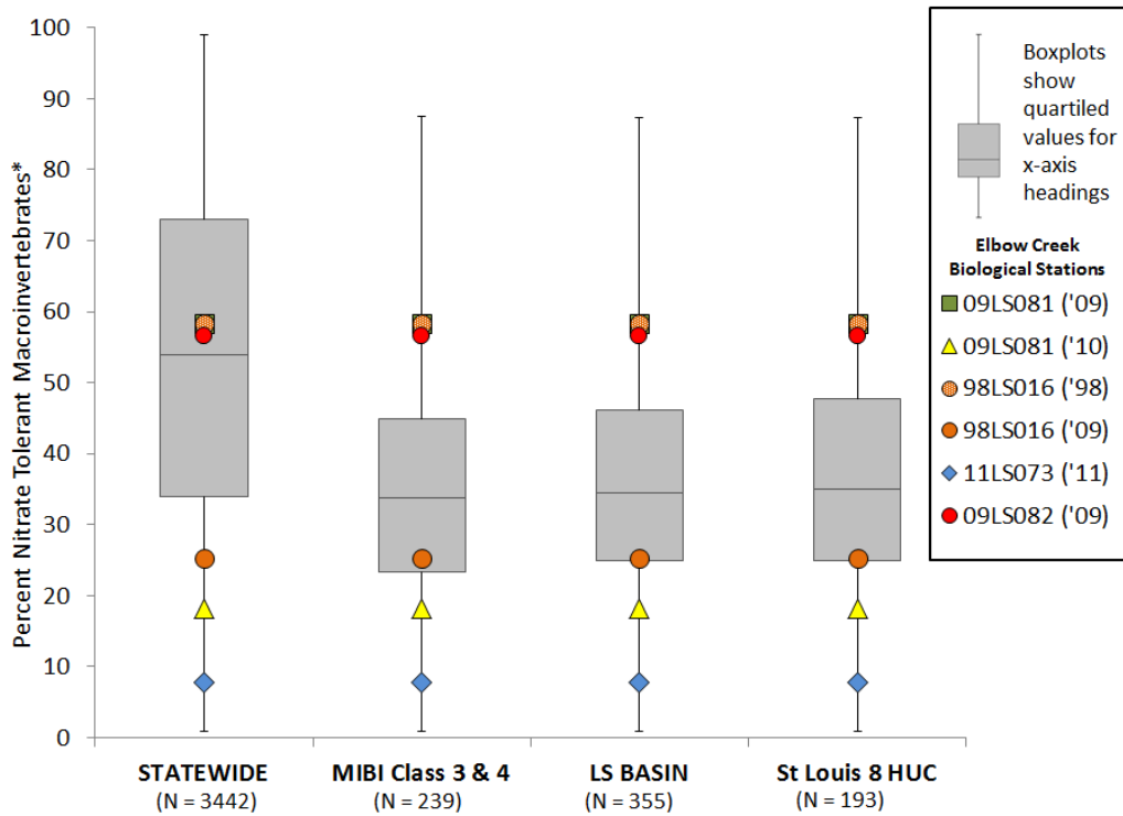
Figure BLANK: Percent nitrate tolerant macroinvertebrates at Elbow Creek monitoring stations compared to statewide and regional monitoring stations
