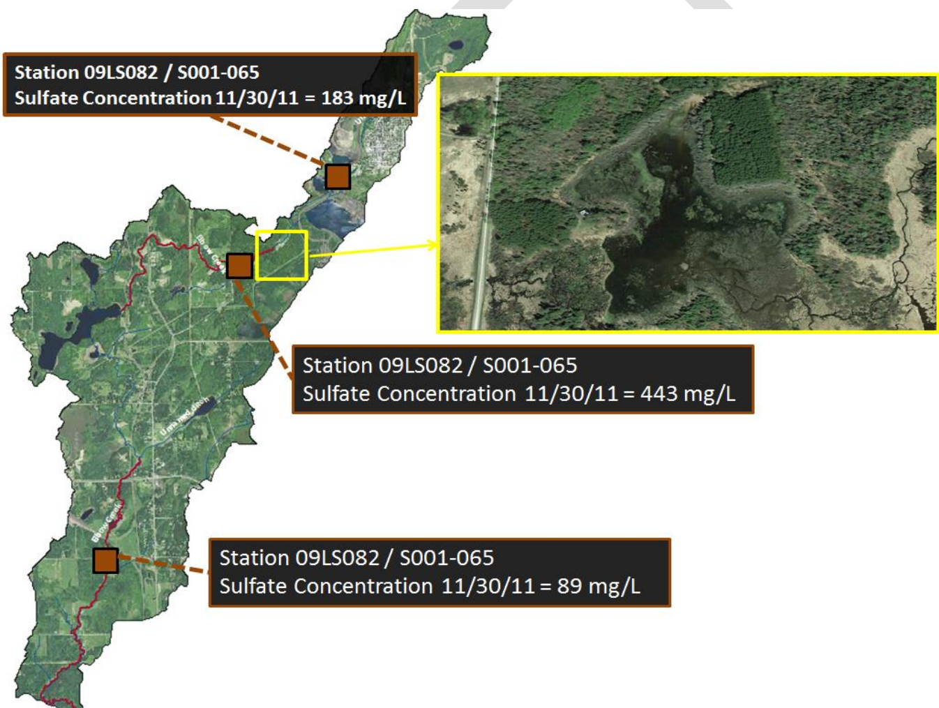
Figure BLANK: Sulfate monitoring results at three locations on Elbow Creek, 11/30/11. A significant increase in sulfate concentration was observed between the two upper monitoring stations where mining waste rock stockpiles are located.
