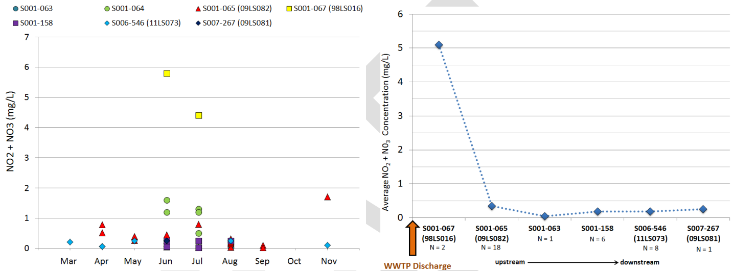
Figure BLANK: Nitrate results from Elbow Creek arranged by monitoring station and month (left). Longitudinal summary of nitrate results showing higher concentrations immediately downstream of Eveleth WWTP (right)
