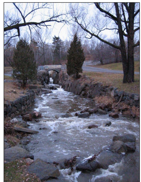
Figure 70: TSS data from Miller Creek near 09LS003, plotted by month (left). Slightly elevated TSS after a fall rain event (right)
