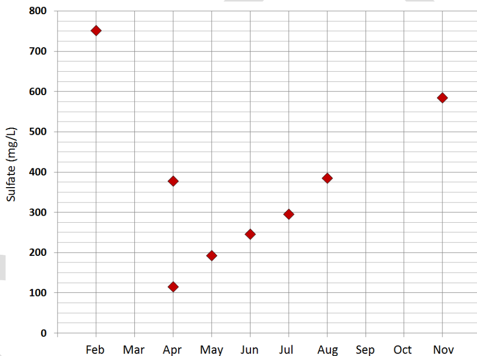
Figure BLANK: Grab sample results for sulfate collected at biological monitoring station 09LS101
