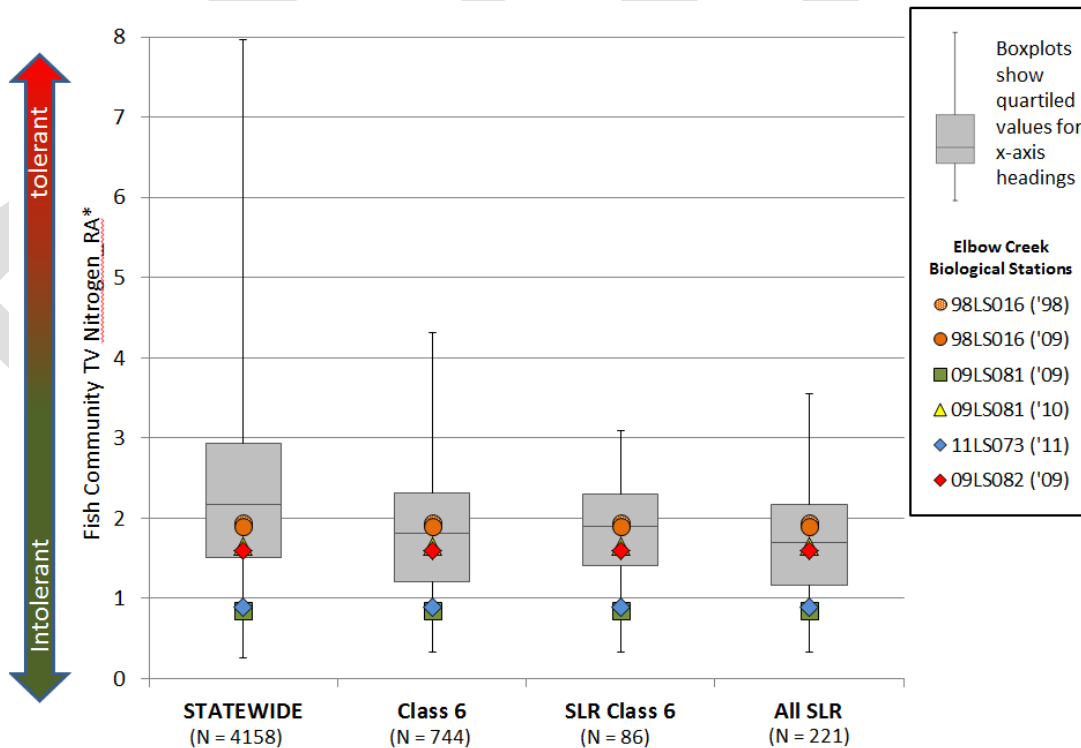
Figure BLANK: Nitrogen tolerance indicator value (NTIV) results for the fish community of Elbow Creek compared to results from statewide and regional monitoring stations
