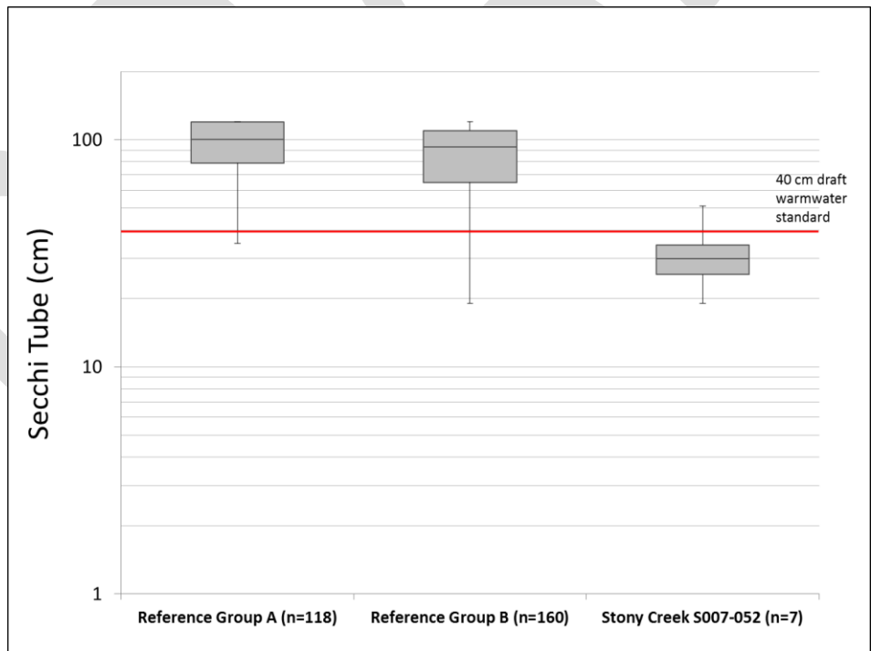
Figure BLANK: Box plots of Secchi tube values for Stony Creek and reference streams
