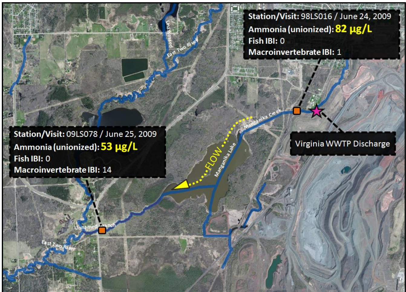
Figure BLANK: Eutrophic conditions in Manganika Lake may be resulting in reduced ammonia concentrations downstream.
