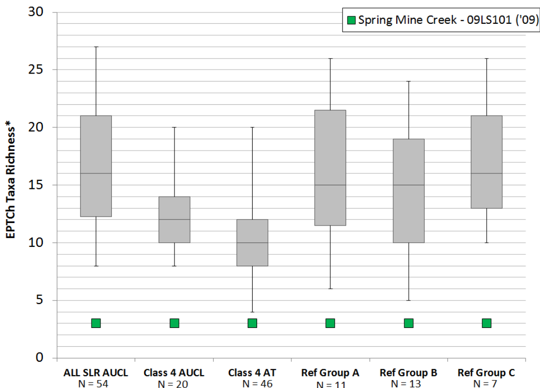
Figure BLANK: EPT taxa richness in Spring Mine Creek compared to high quality SLRW reference stations
