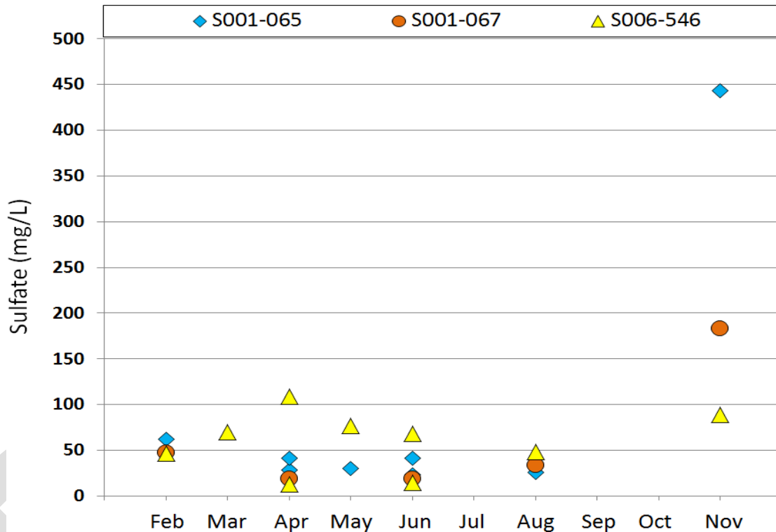
Figure BLANK: All available sulfate data from Elbow Creek. Data collected in 2011, 2012, and 2014.
