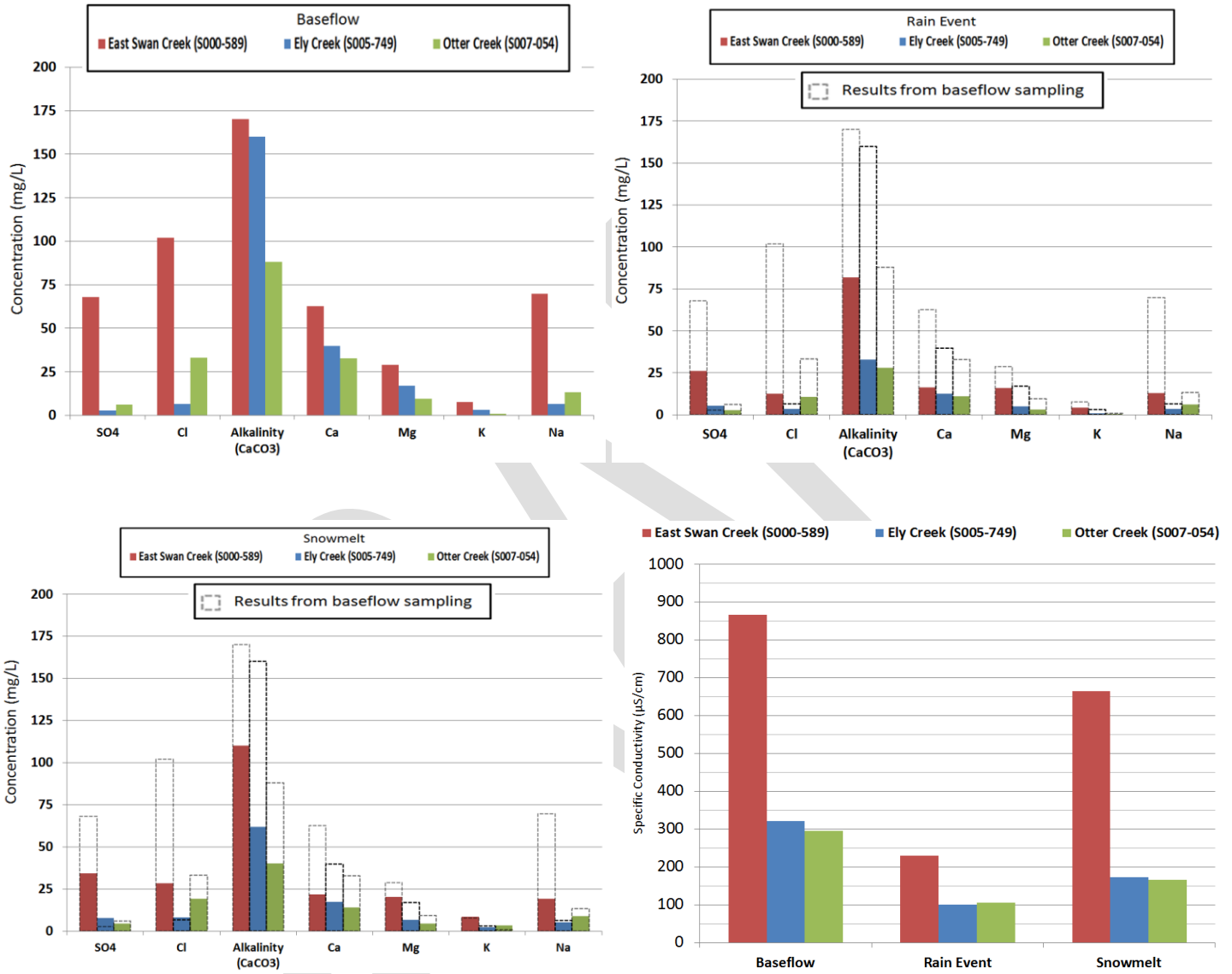
Figure BLANK: Comparison of geochemistry sampling results for major cations and anions in East Swan Creek, Ely Creek, and Otter Creek under various flow conditions; baseflow (upper left), rain event (upper right), snowmelt (lower left). Specific conductivity comparisons for East Swan Creek, Ely Creek, and Otter Creek during the same sampling events (lower right).
