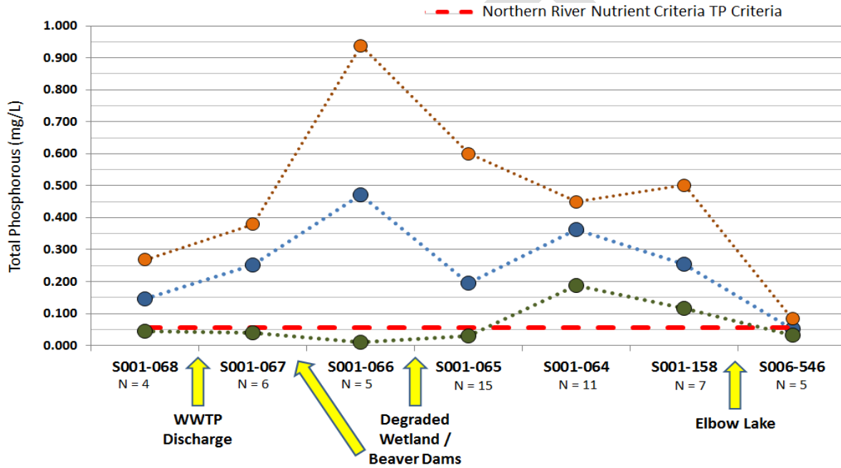
Figure BLANK: Minimum, average, and maximum total phosphorous concentrations observed at Elbow Creek monitoring stations.
