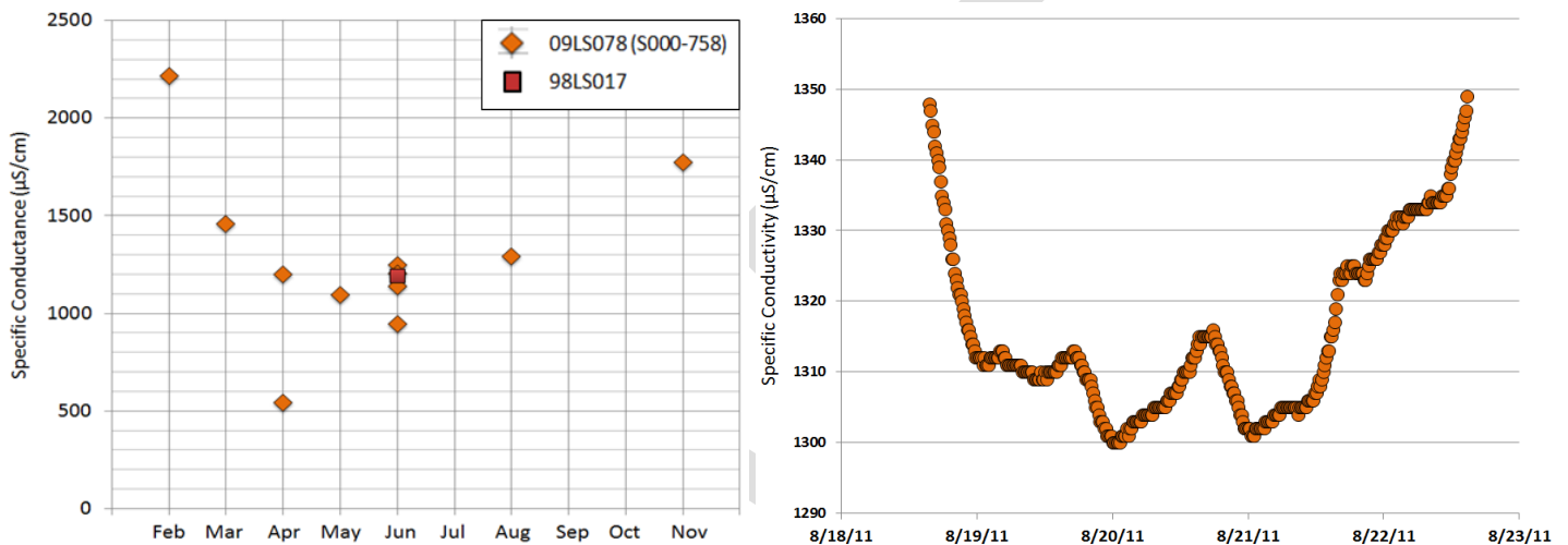
Figure BLANK: Point measurements of specific conductivity (left) and conductivity levels during a 5-day continuous monitoring period at biological monitoring station 09LS078
