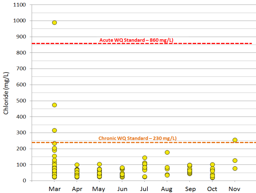
Figure 54: Kingsbury Creek chloride grab sampling results arranged by calendar month (all monitoring sites combined).
