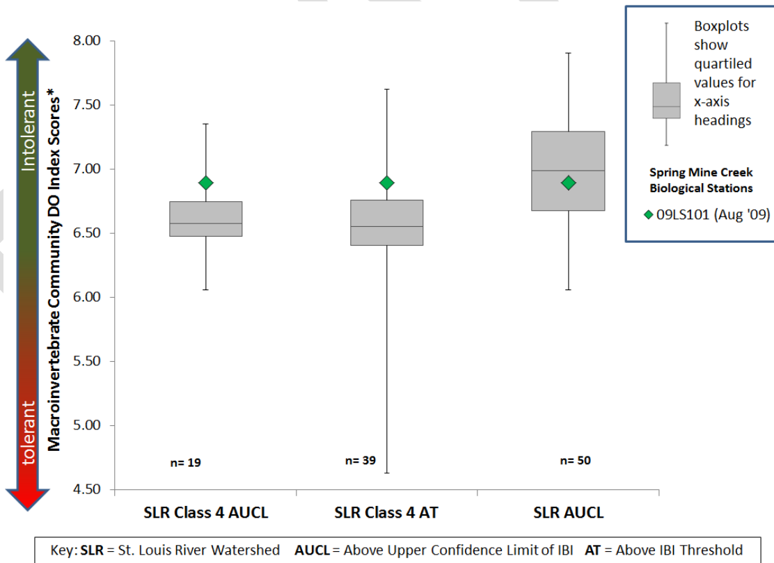
Figure BLANK: Macroinvertebrate community DO TIV results for Spring Mine Ck vs. high quality stations of the same IBI class
