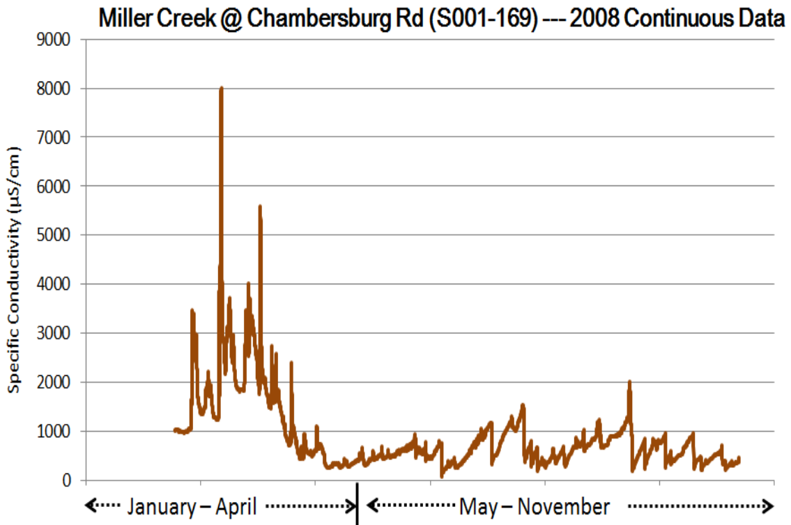
Figure 82: Continuous specific conductivity data collected at station S001-169 in 2008
