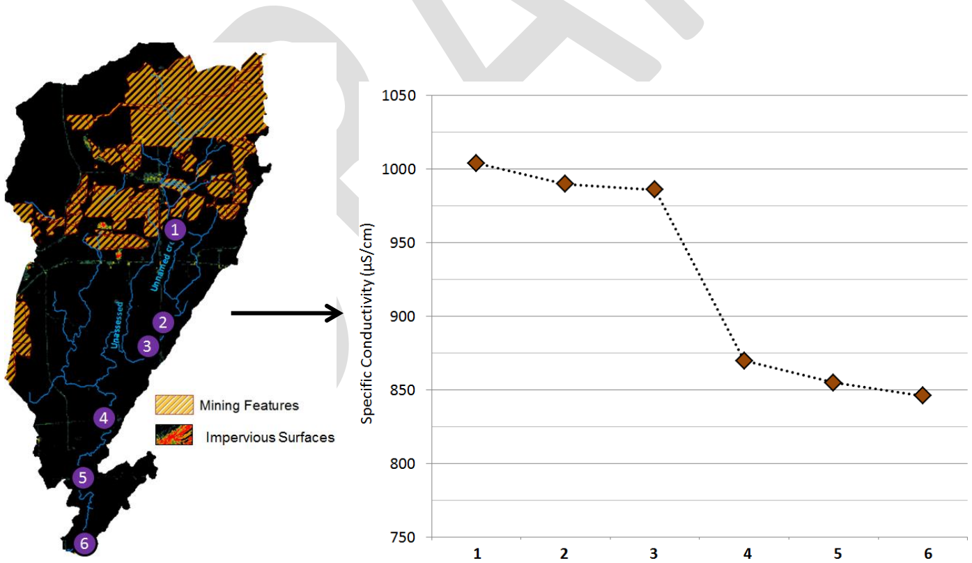
Figure BLANK: Longitudinal specific conductivity results from Kinney Creek; September 2014
