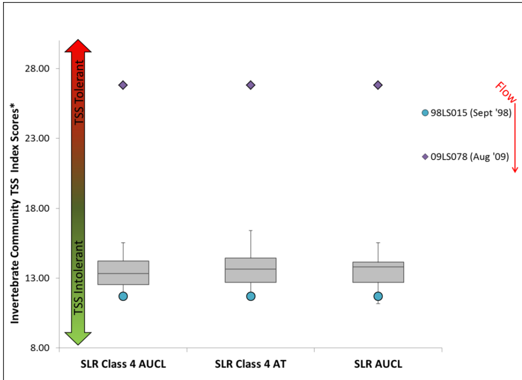
Figure BLANK: Macroinvertebrate community TSS TIVs for Manganika Creek, compared to unimpaired streams
