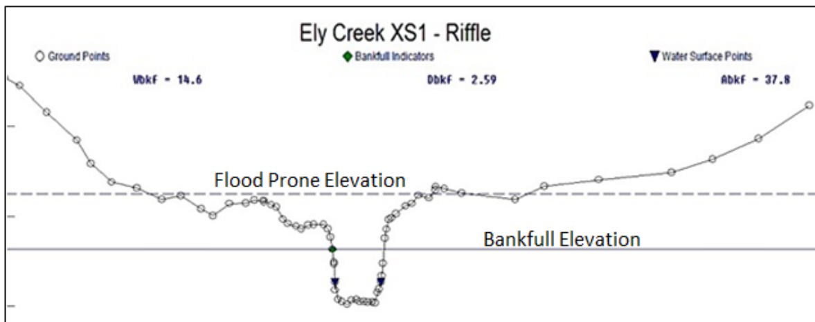
Figure BLANK: Survey data from riffle cross-section at station 09LS084 showing channel incision
