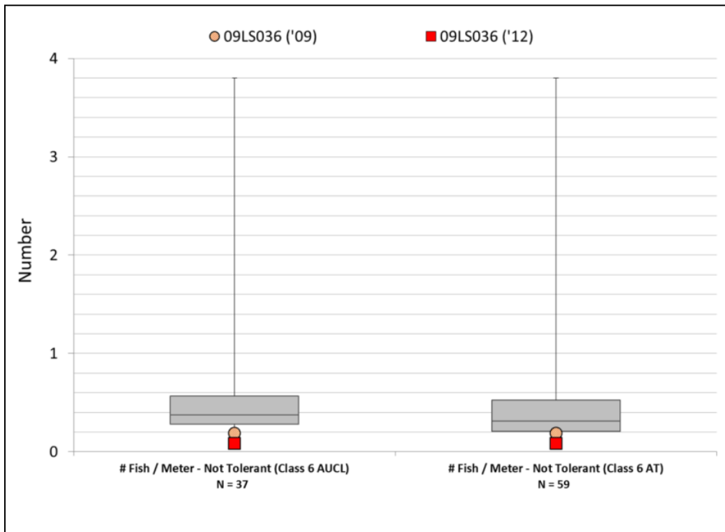
Figure BLANK: Non-tolerant fish/meter in Stony Creek compared to high quality Class 6 SLRW stations
