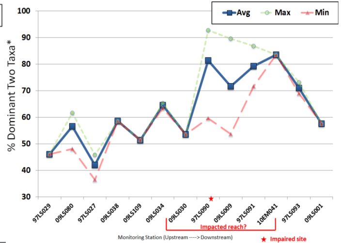
Figure BLANK: A series of macroinvertebrate metric data showing a decline in biological integrity within and around the impaired reach of the St. Louis River
