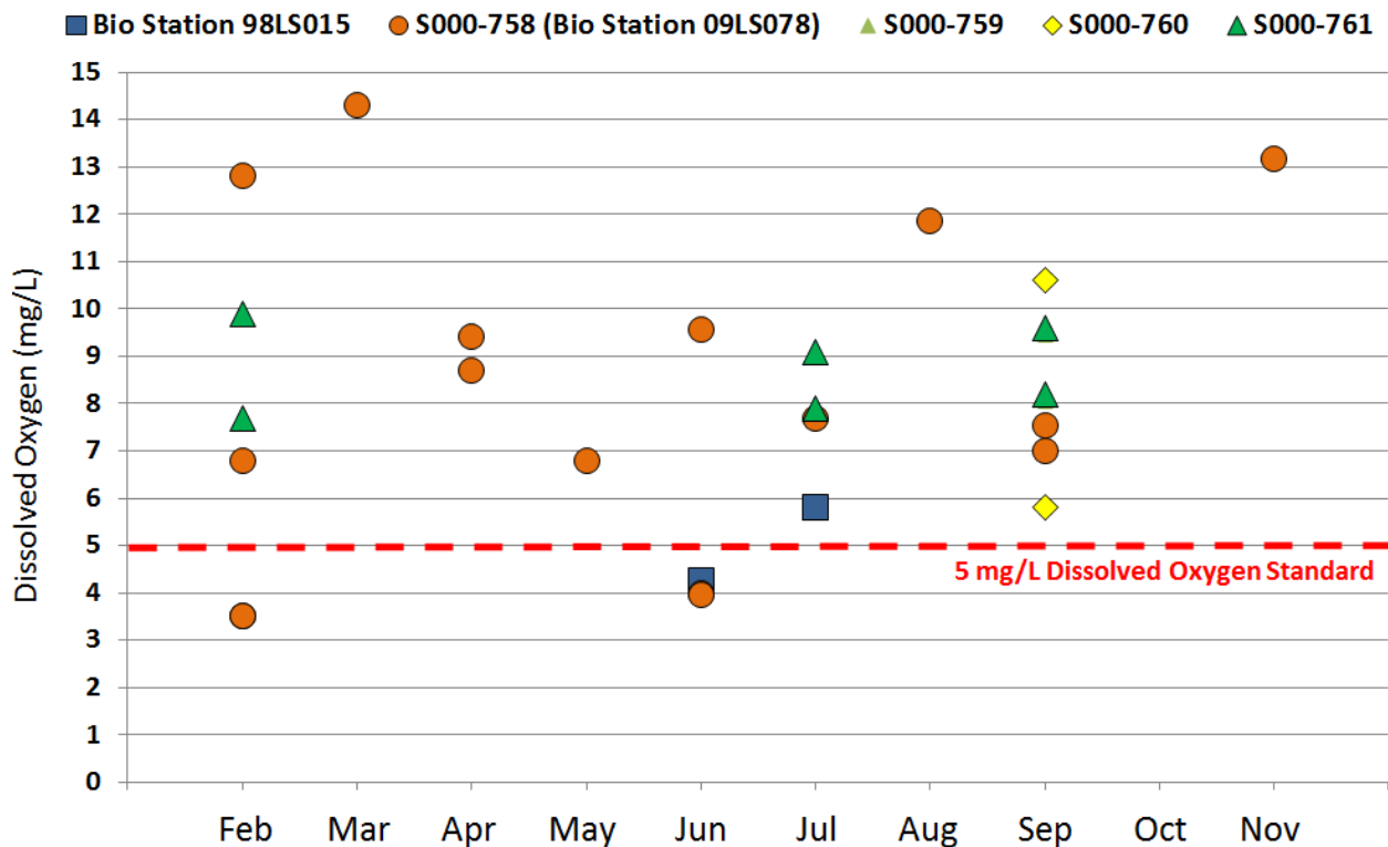
Figure BLANK: Point measurements of dissolved oxygen collected from Manganika Creek
