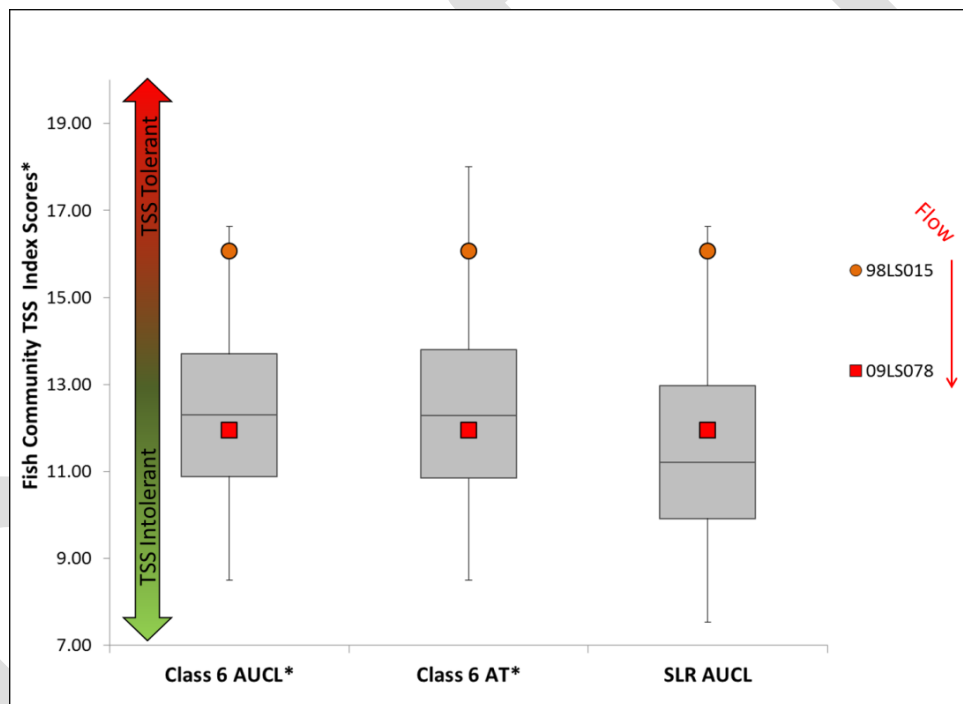
Figure BLANK: Fish community TSS TIVs for Manganika Creek, compared to unimpaired streams
