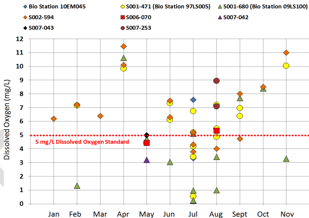
Figure BLANK: Point measurements of dissolved oxygen collected within the impaired reach of the Embarrass River plotted by monitoring station and calendar month.
