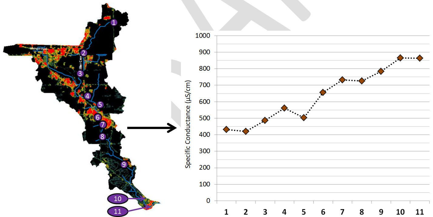
Figure 84: Results from longitudinal specific conductivity monitoring conducted September 12, 2014
