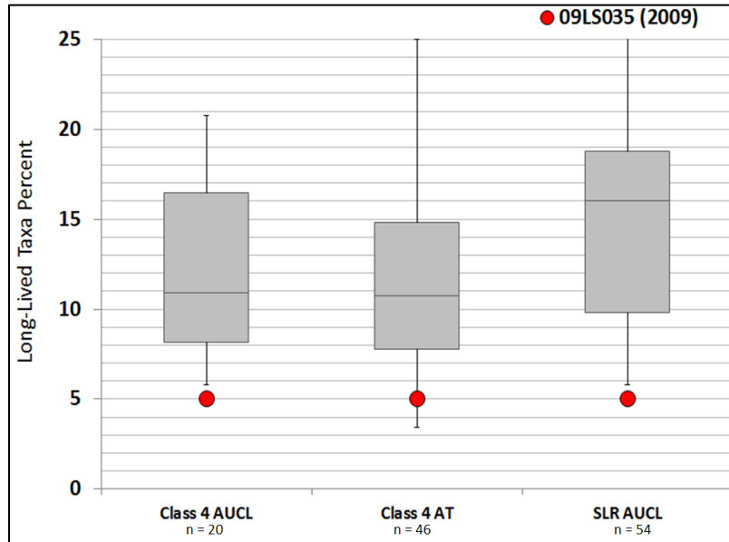
Figure BLANK: Long-lived macroinvertebrate taxa percent observed at station 09LS035 compared to high quality reference stations
