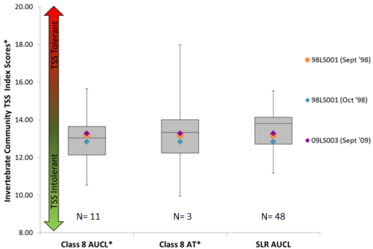
Figure 75: Macroinvertebrate community TSS TIVs for Miller Creek, compared to unimpaired streams (* see table blank)
