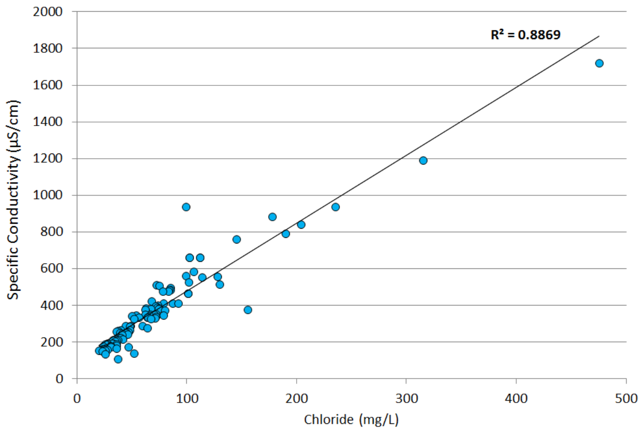
Figure 60: Scatter-plot regression of paired chloride and specific conductivity measurements from Kingsbury Creek
