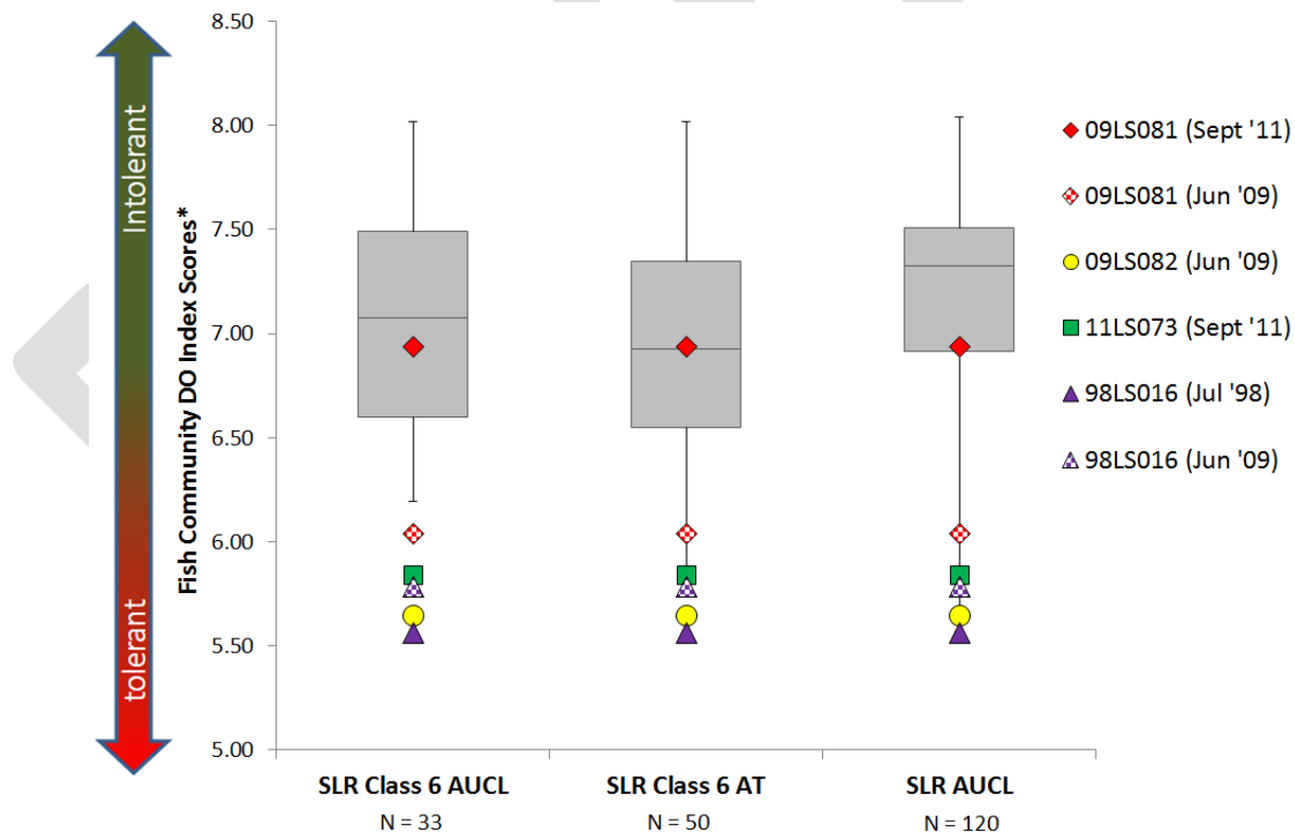
Figure BLANK: Fish community DO TIV results for Elbow Creek monitoring sites compared to high quality reference stations
