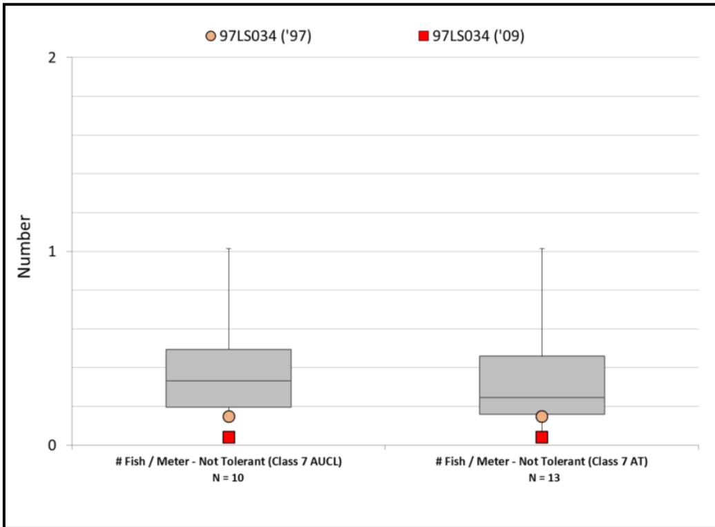
Figure BLANK: Non-tolerant fish/meter in Vaara Creek compared to high quality Class 7 SLRW stations
