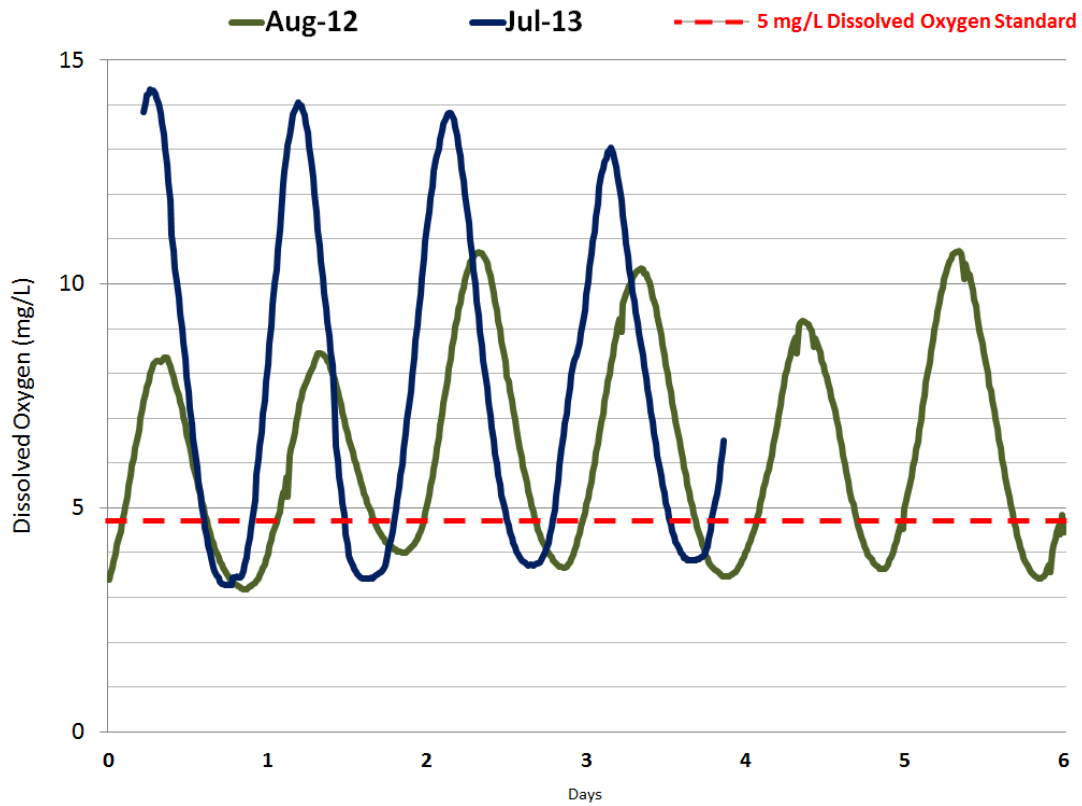
Figure BLANK: Results of continuous dissolved oxygen monitoring at station 09LS075 in August 2012 and July 2013
