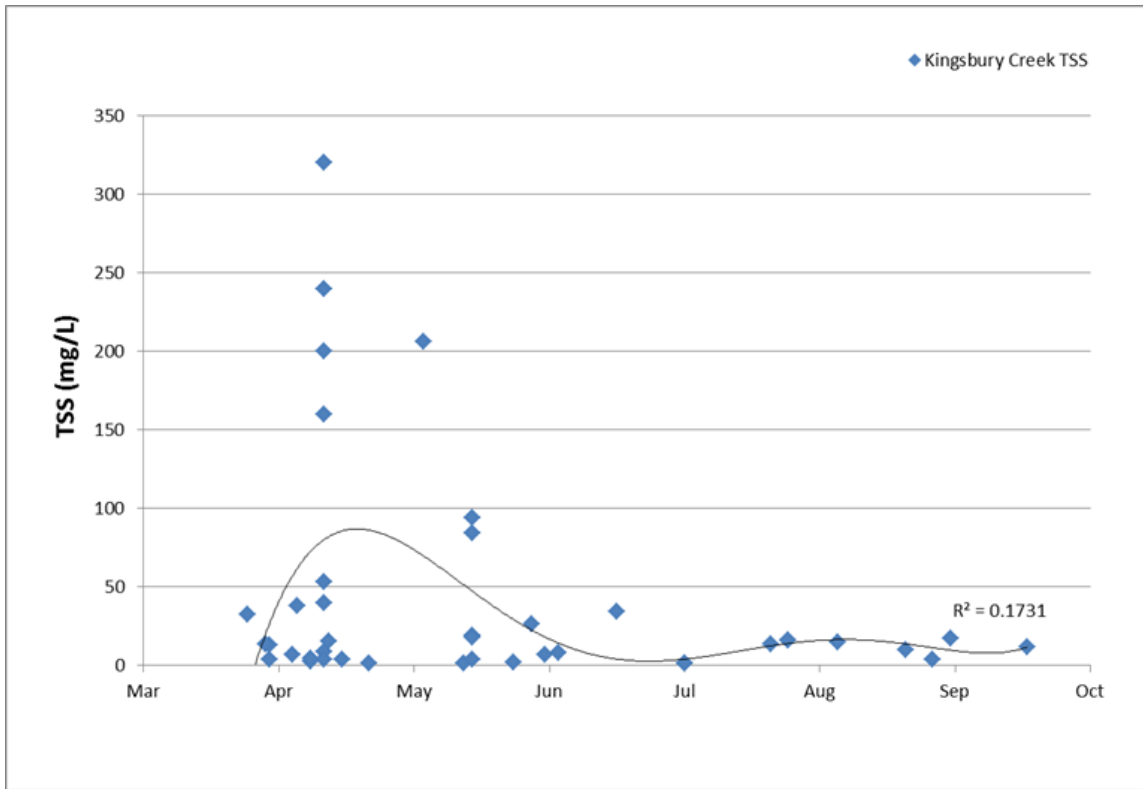
Figure 43: TSS results for Kingsbury Creek by month
