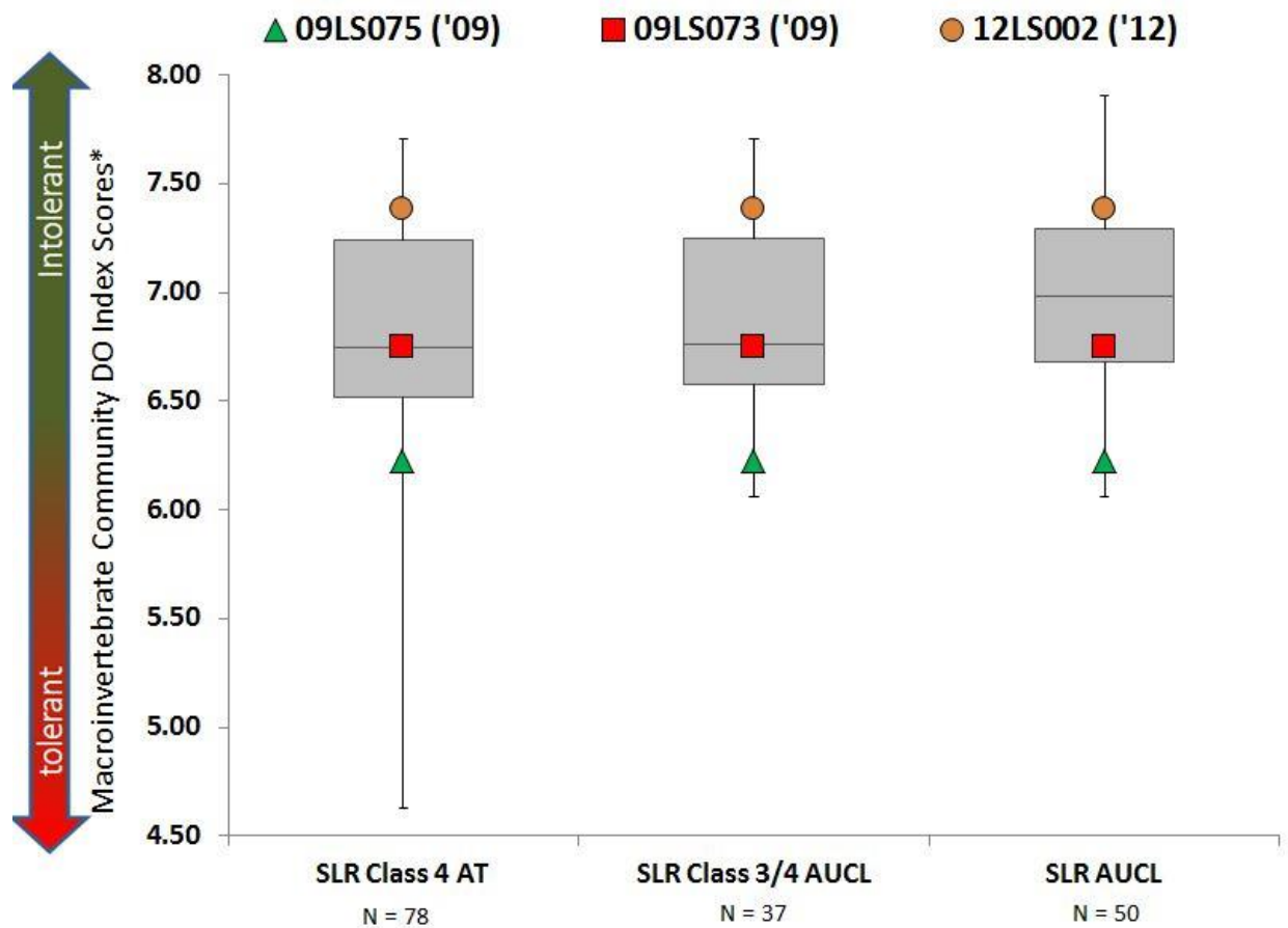
Figure BLANK: Macroinvertebrate community tolerance indicator values (TIV) for dissolved oxygen at West Two River monitoring sites compared to non-impaired streams in the SLRW
