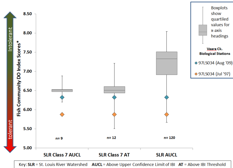
Figure BLANK: Fish community dissolved oxygen TIV results for Vaara Creek compared to high quality reference stations
