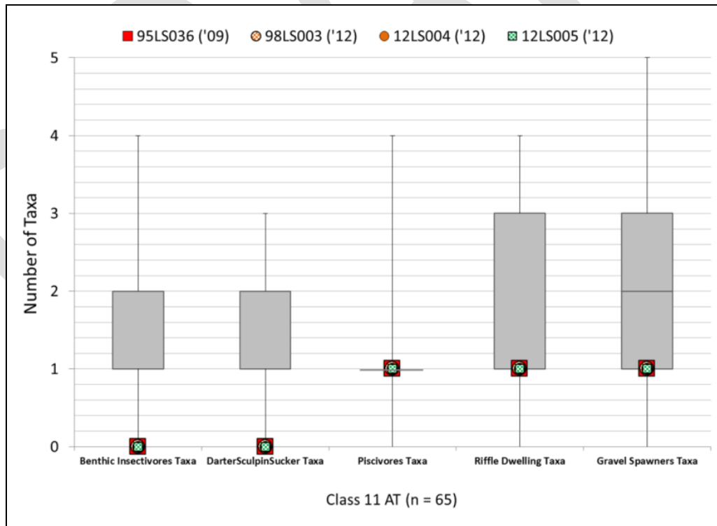
Figure 63: Number of fish taxa for various categories in Kingsbury Creek compared to SLRW stations above the impairment threshold
