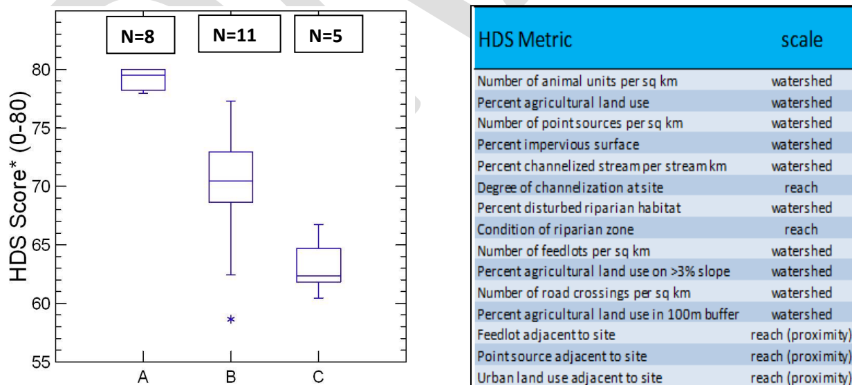
Figure 9: Box plot summary of human Disturbance Gradient (HDS) scores for the three water quality reference station classes (left) and list of metrics used to develop the HDS score (right)
