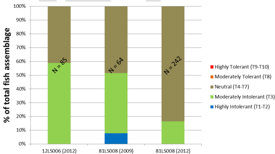
Figure BLANK: TSS tolerance of fish assemblages by site in Wyman Creek (n = number of fish)
