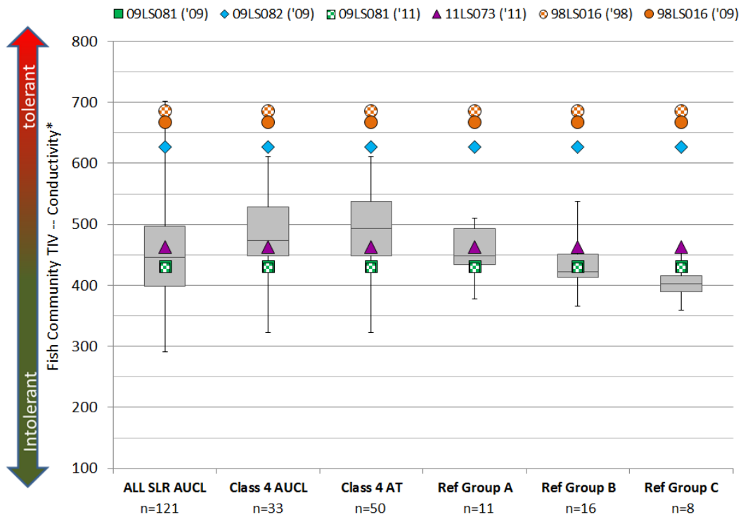
Figure BLANK: Community level TIV values for specific conductivity in Elbow Creek compared to SLRW reference sites
