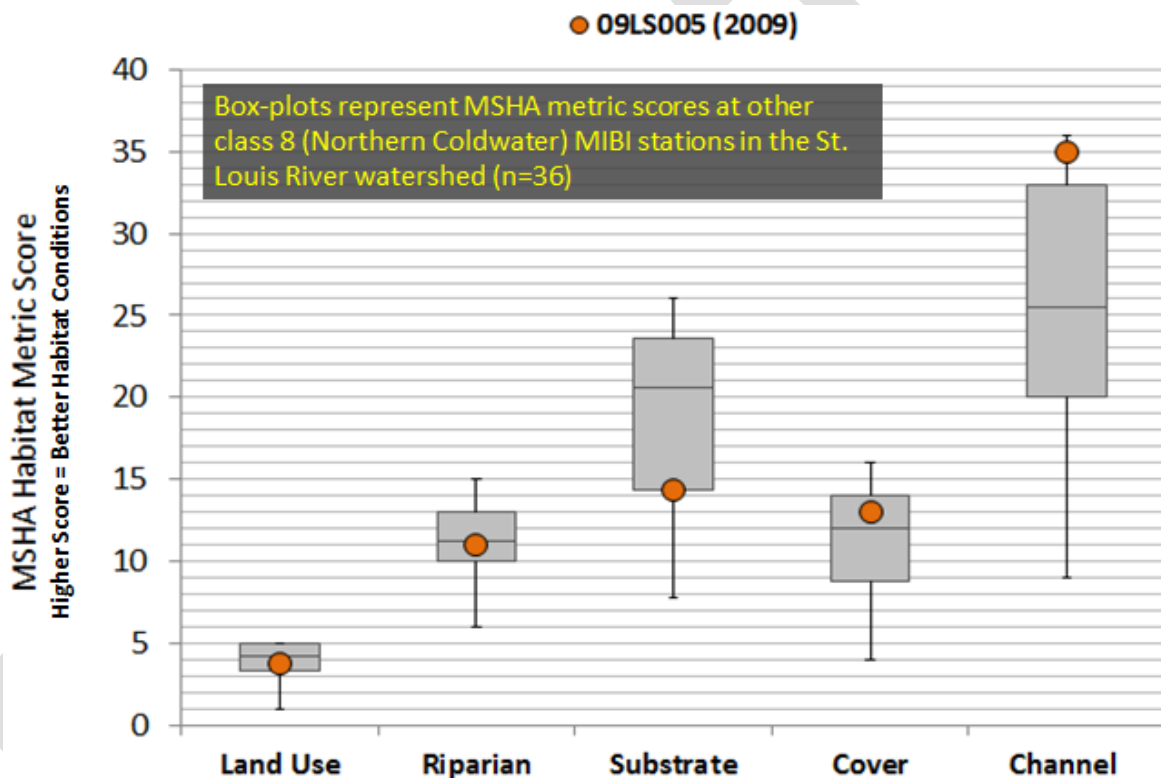
Figure BLANK: Minnesota Stream Habitat Assessment (MSHA) metric scores for Otter Creek station 09LS005 compared to the box plot distribution of results from all other class 8 (Northern Coldwater) stations in the St. Louis River Watershed.
