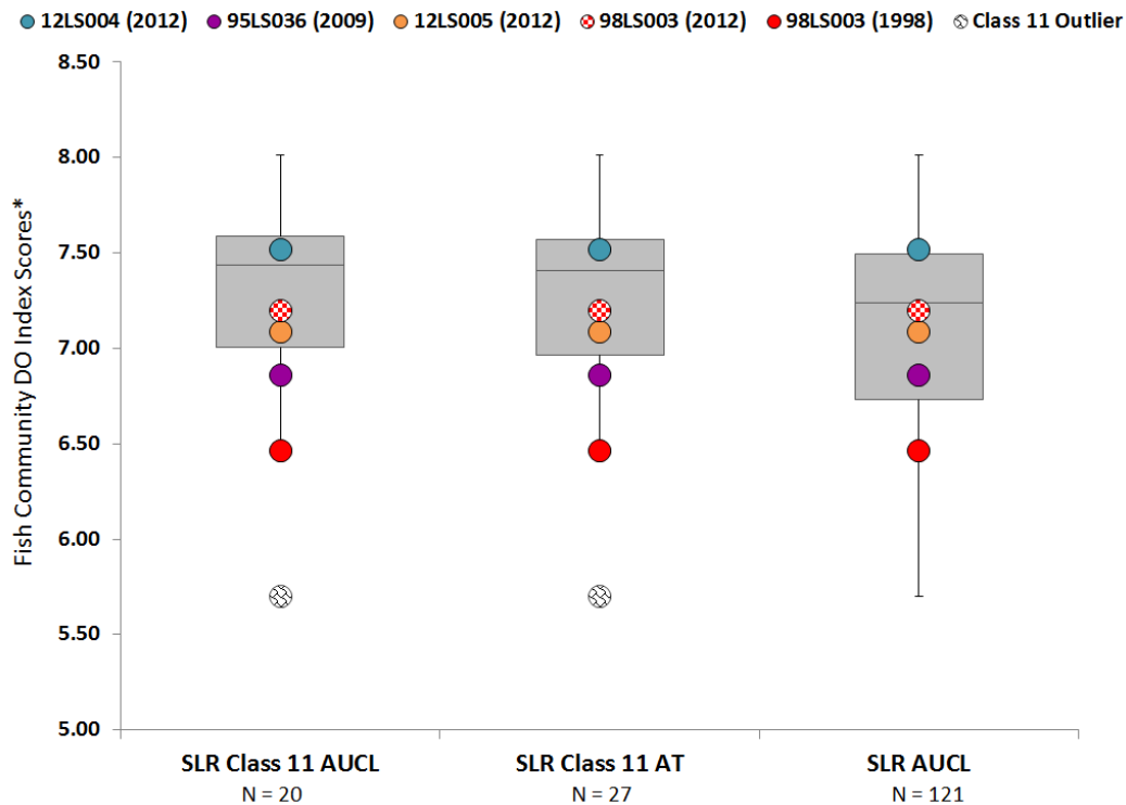
Figure 38: Fish community DO TIV results for Kingsbury Creek compared to high quality stations (*see table blank for acronym descriptions)
