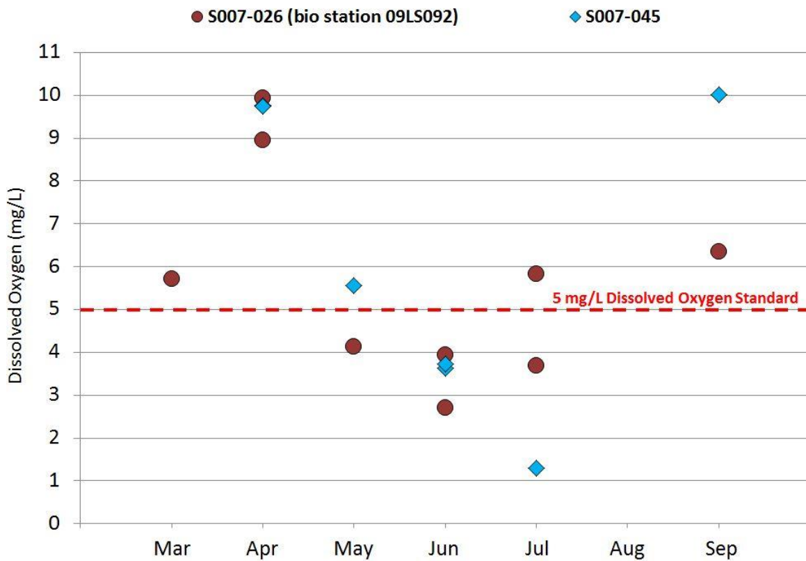
Figure BLANK: Point measurements of dissolved oxygen collected on Water Hen Creek / Water Hen River.
