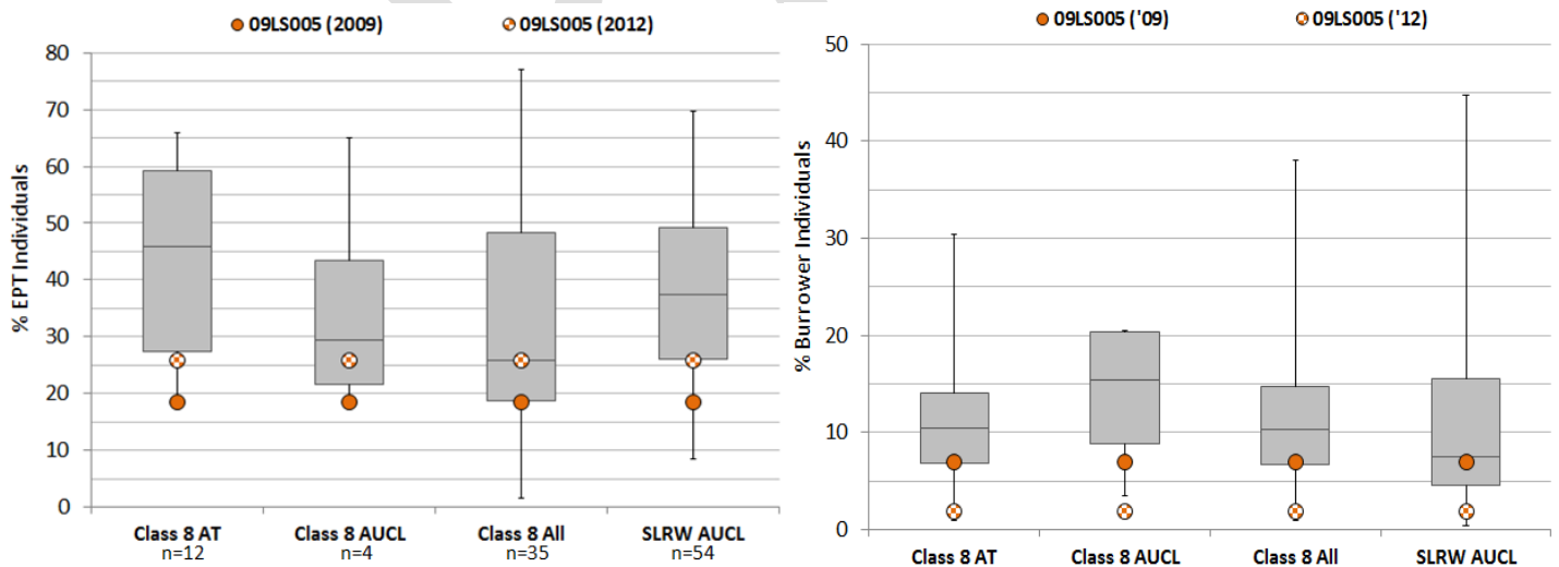
Figure BLANK: % EPT individuals (left) and % burrower individuals (right) observed at Otter Creek 09LS005 compared results from various groupings of SLRW stations. See appendix BLANK for category descriptions.
