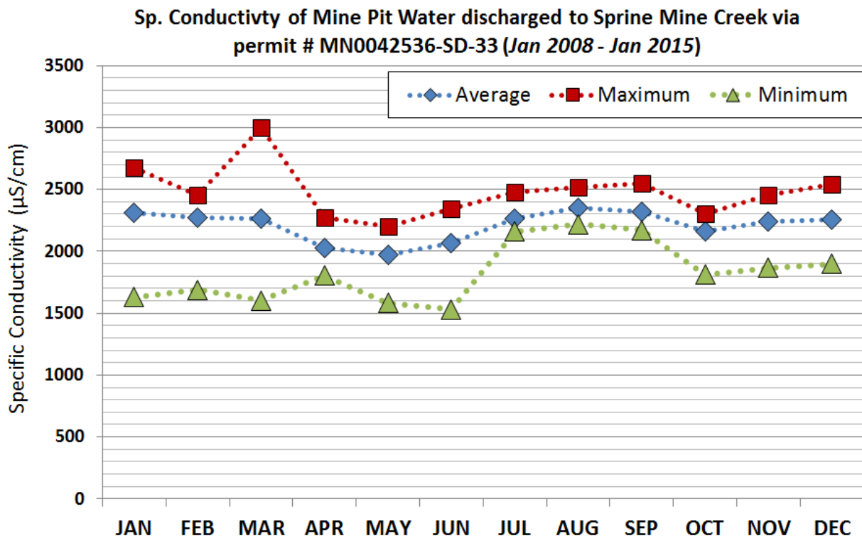
Figure BLANK: Continuous specific conductivity data collected at the outlet of the abandoned mine pit that serves as the headwaters of Spring Mine Creek.
