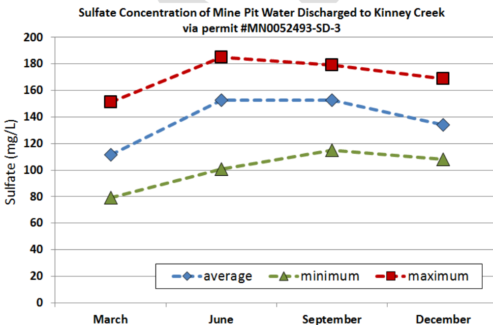
Figure BLANK: Summary of sulfate concentrations observed in the mine pit water pumped into Kinney Creek via permit MN0052493-SD-3. Monitoring data are from samples collected each March, June, September, and December from 2004 through 2014.
