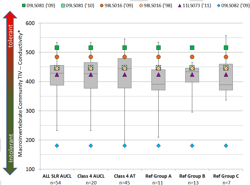
Figure BLANK: Community level TIV values for specific conductivity in Elbow Creek compared to SLRW reference sites
