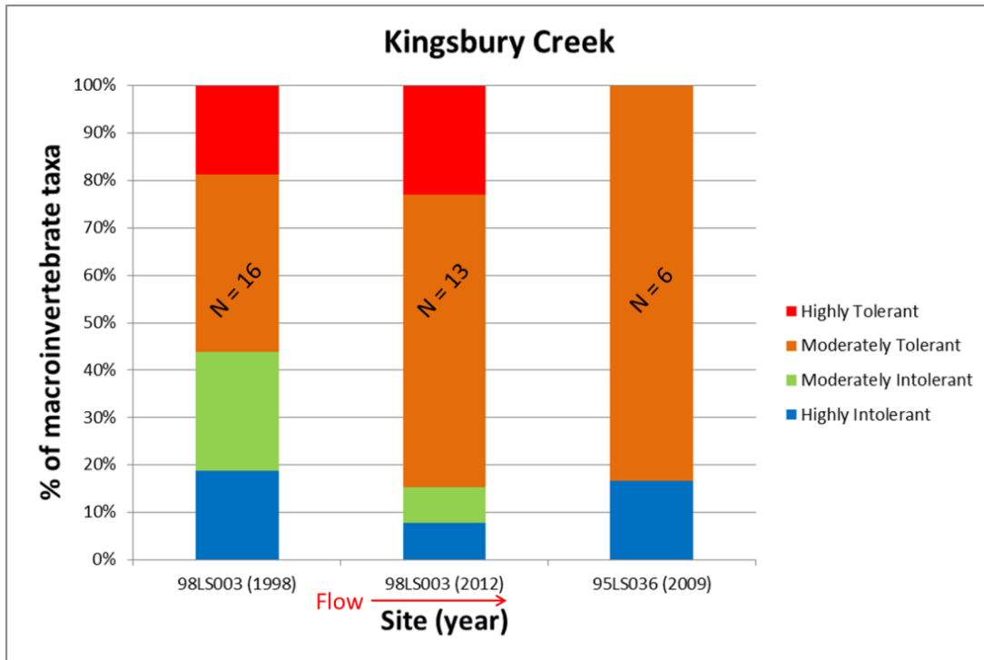
Figure 52: TSS tolerance of macroinvertebrate assemblages by site in Kingsbury Creek (n = number of taxa)
