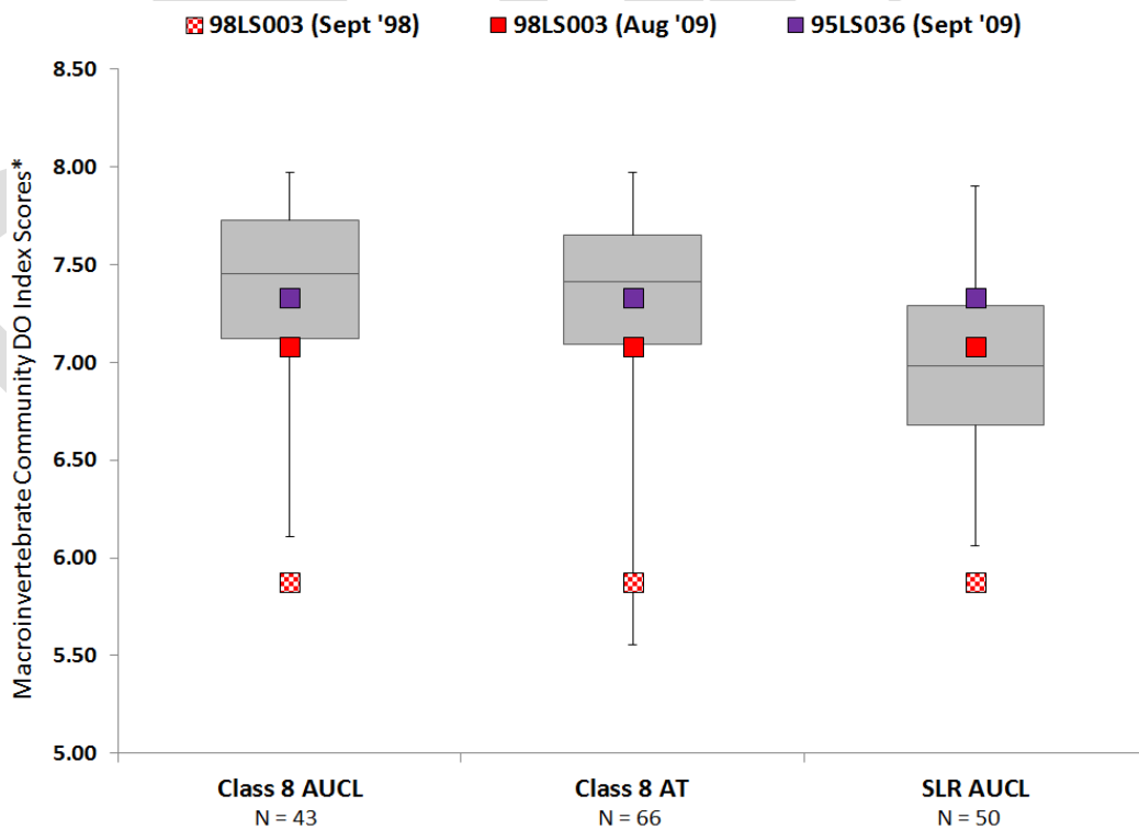
Figure 39: Macroinvertebrate community DO TIV results for Kingsbury Creek compared to high quality stations (*see table blank for acronym descriptions)
