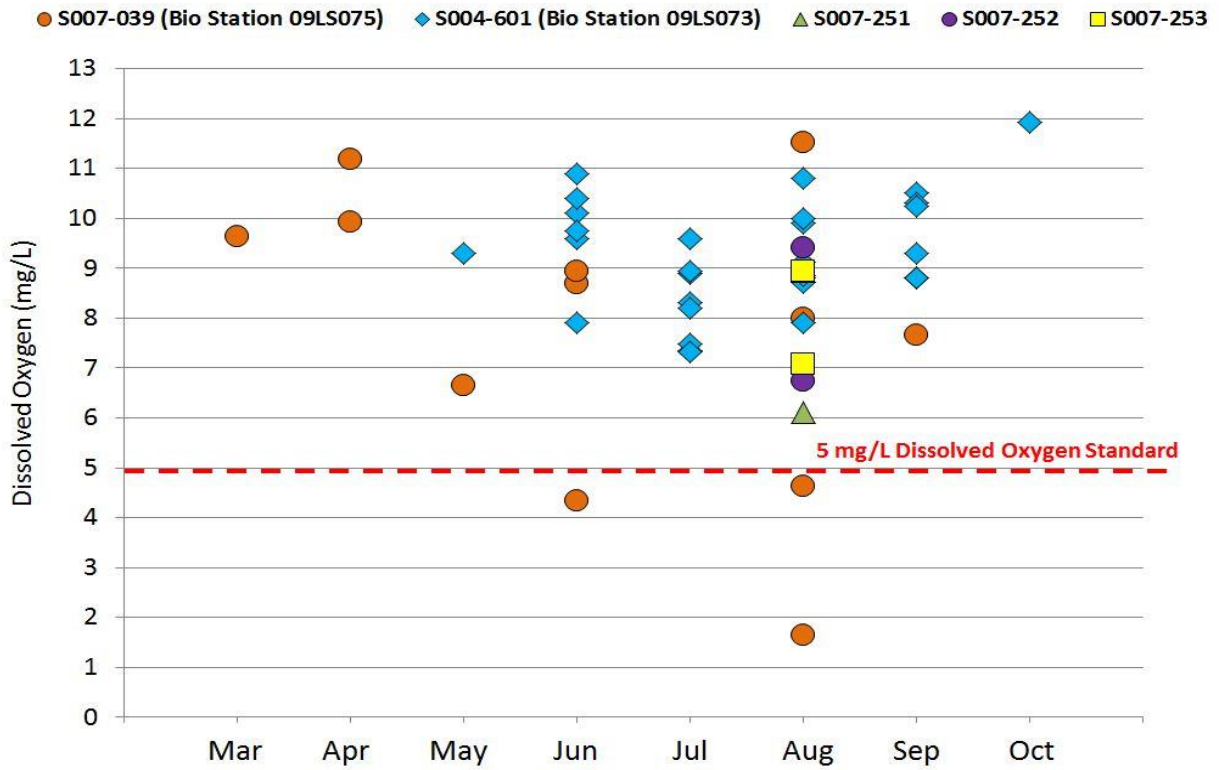
Figure BLANK: Point measurements of dissolved oxygen collected from the West Two River
