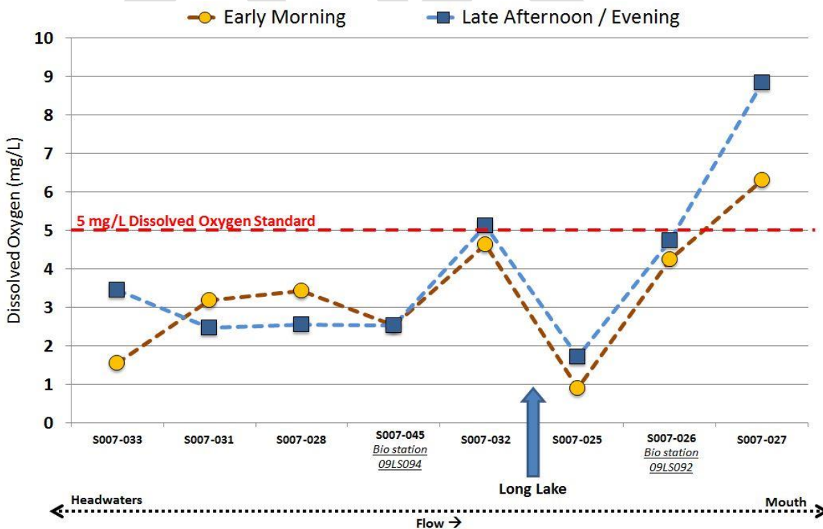
Figure BLANK: Results from the 7/29/2011 longitudinal synoptic dissolved oxygen profile.
