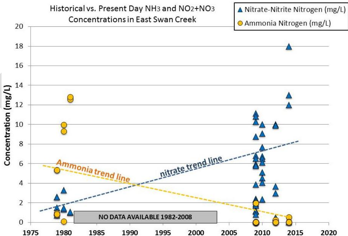
Figure BLANK: Comparison of historic and contemporary ammonia and nitrate nitrogen data collected from East Swan Creek
