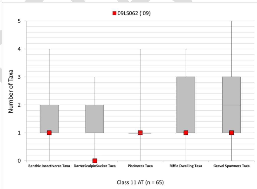
Figure 4: Number of fish taxa for various categories in Little Swan Creek compared to SLRW stations above the impairment threshold
