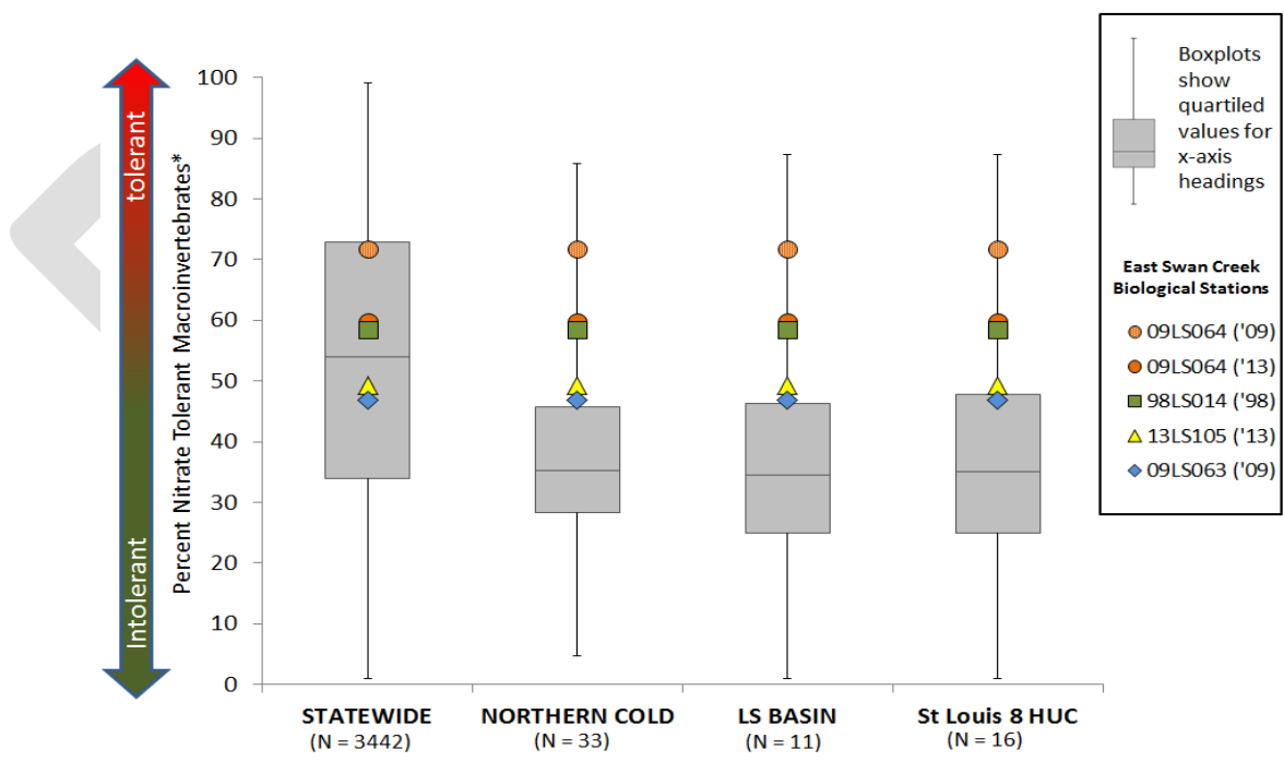
Figure BLANK: Percent nitrate tolerant macroinvertebrates observed at East Swan Creek monitoring stations compared to results from statewide and regional sites
