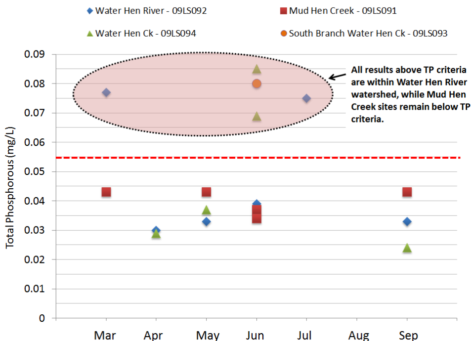
Figure BLANK: Total phosphorous (TP) results for Water Hen Creek and Mud Hen Creek watershed
