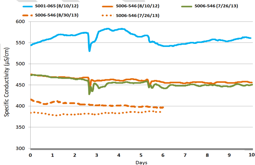
Figure BLANK: Continuous specific conductivity results measured over a 6-10 day period at several Elbow Creek monitoring sites
