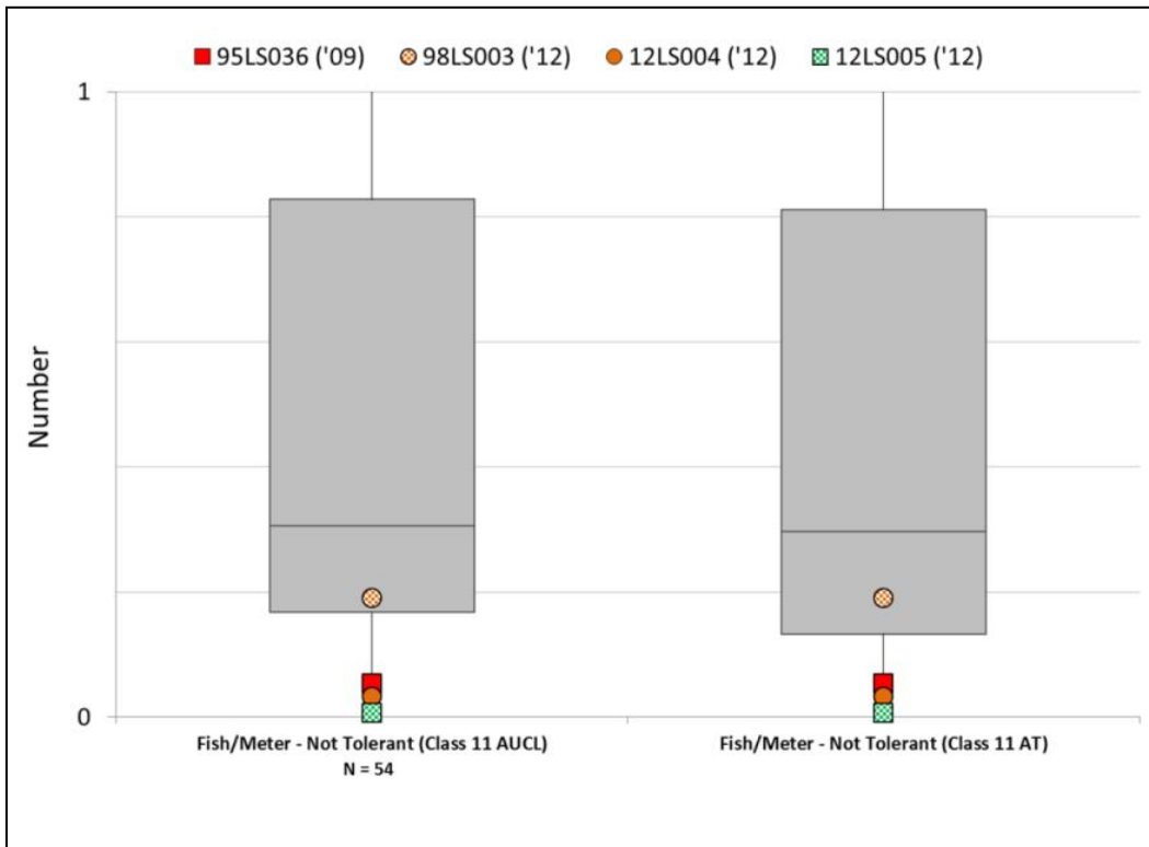
Figure 62: Fish/meter (excluding tolerant taxa) in Kingsbury Creek compared to high quality SLRW Class 11 stations
