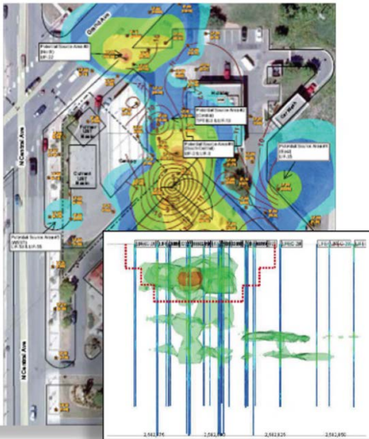
Bay West used state-of-the-art ultraviolet optical screening tools to characterize underground contamination.
