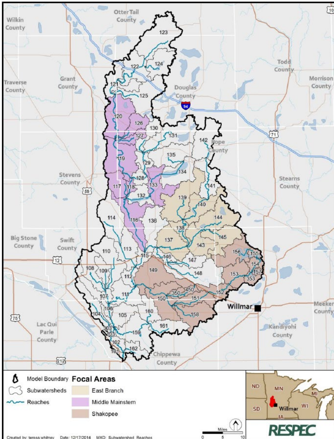
Figure 2. HSPF Subwatersheds and Reaches.
