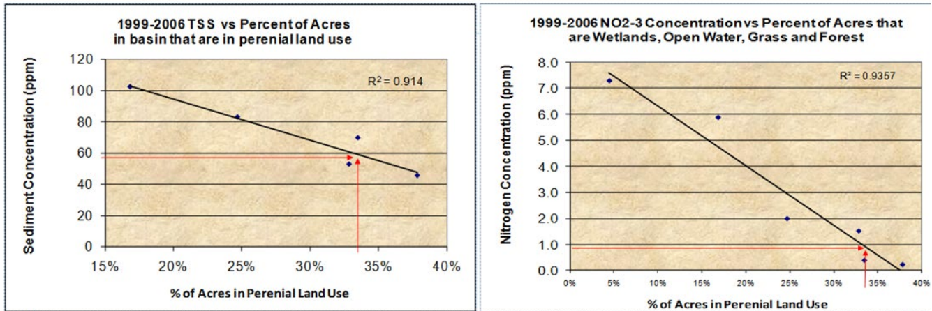
Figure 37: CRWP correlation of land cover to average flow weighted mean
