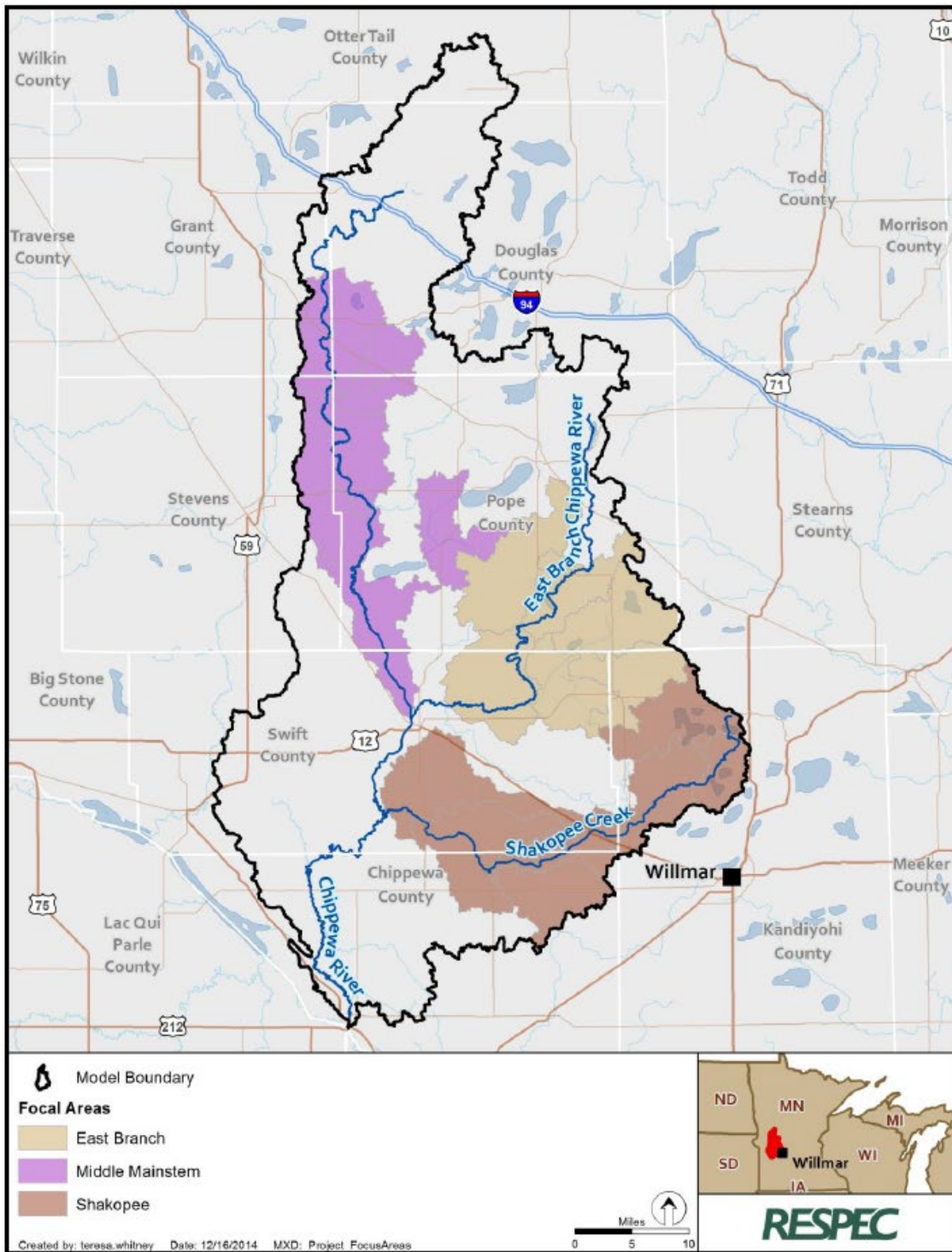
Figure 1. HSPF Model Boundary and Focal Areas.
